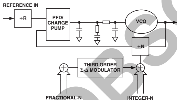
Figure 11. Fractional-N PLL
