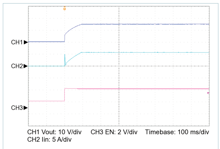
Figure 14 — Startup from EN, V_{IN} = 30\text{ V} , C_{OUT\_EXT} = 10000\text{ }\mu\text{F} , R_{LOAD} = 1.402\text{ }\Omega
