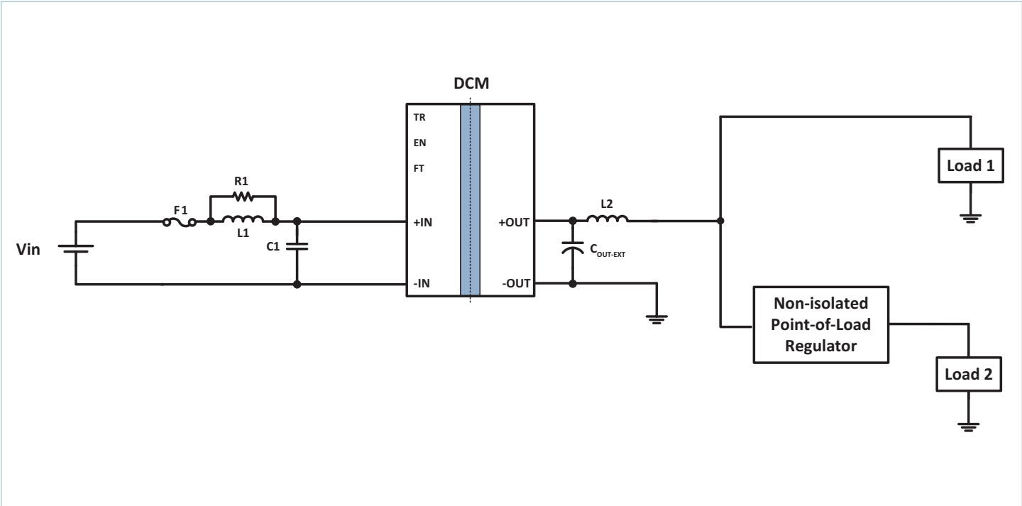
Typical Application: Single DCM3623x50T17A6y7z, to a non-isolated regulator, and direct to load
