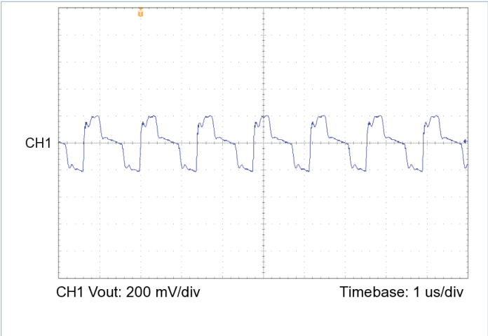
Figure 16 — Output voltage ripple, V_{IN} = 30\text{ V} , V_{OUT} = 15.0\text{ V} , C_{OUT\_EXT} = 1000\text{ }\mu\text{F} , R_{LOAD} = 1.402\text{ }\Omega
