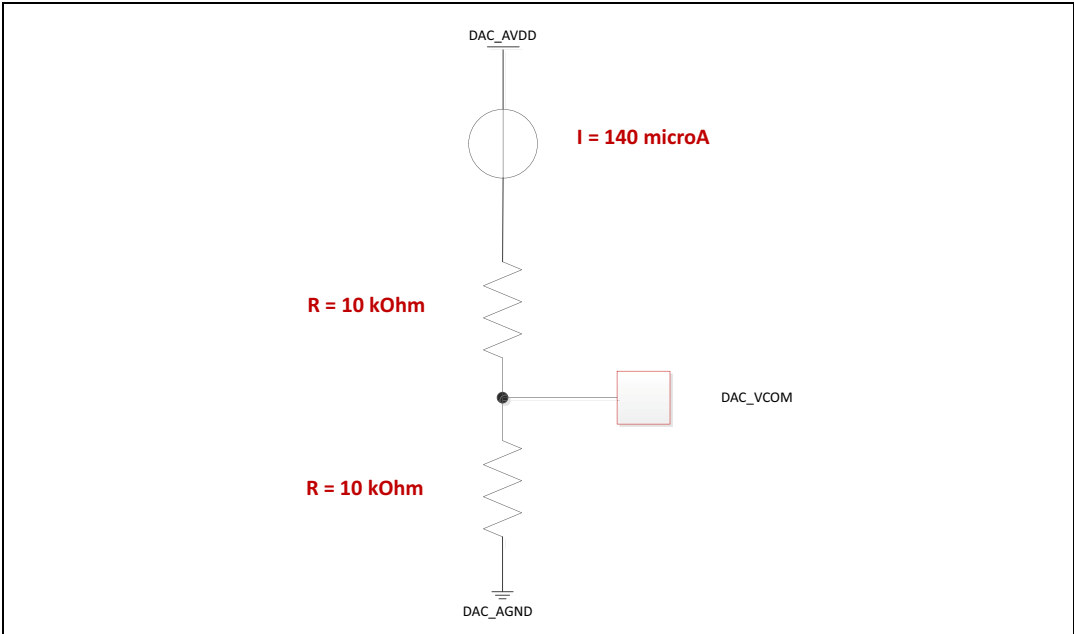
Figure 10. DAC VCOM Equivalent Circuit
