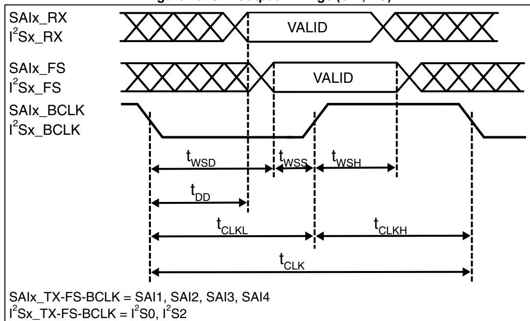
Figure 20. SAI Output Timings (SAI, I 2 S)
