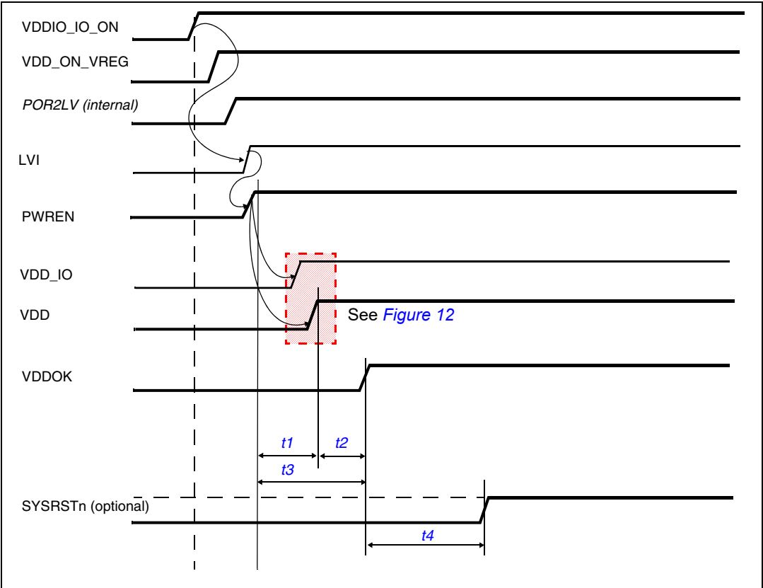
Figure 13. Initial Power-On Sequence (VDDOK timed)
