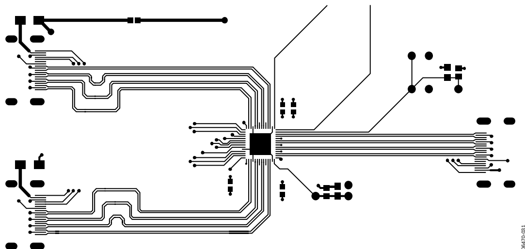
Figure 31. Evaluation Board Layout of the TMDS Traces
