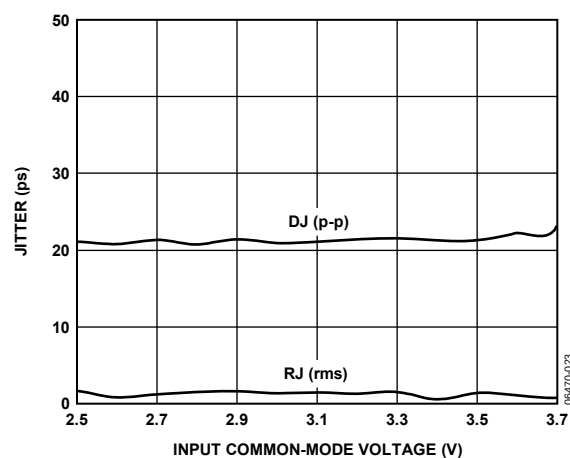
Figure 23. Jitter vs. Input Common-Mode Voltage
