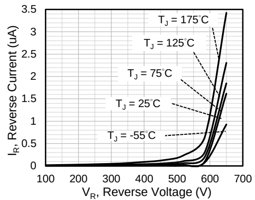
Fig.2 Reverse Characteristics
