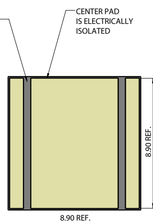
Alternate Bottom View
