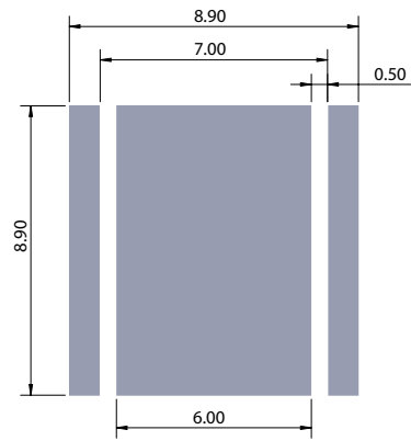
Recommended PCB Footprint
