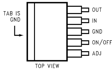
TO-263 (KTT) Surface-Mount Package 4 Pins Top View
