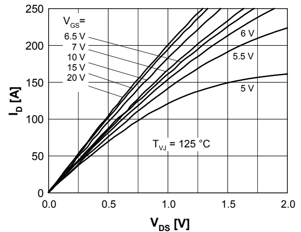
Fig. 4 Typ. output characteristics (125 °C)
