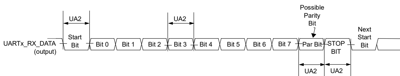
Figure 47. UART RS-232 Serial mode receive timing diagram
