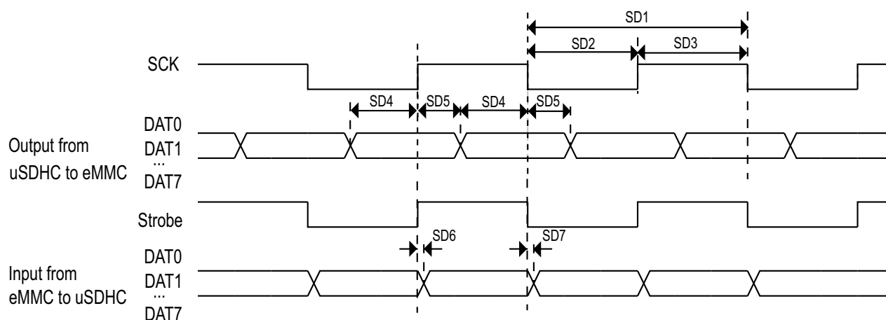
Figure 15. HS400 timing
