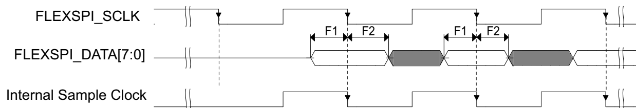
Figure 35. FlexSPI input timing in SDR mode where FlexSPI n _MCR0[RXCLKSRC] = 0x0, 0x1
