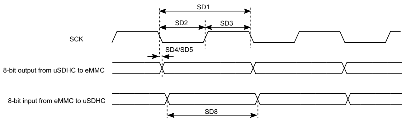
Figure 16. HS200 timing
