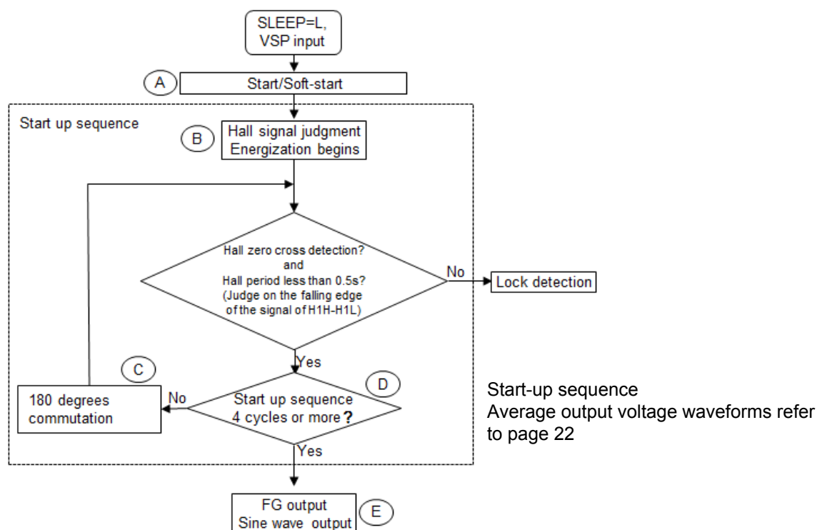
Start-up sequence flow chart
