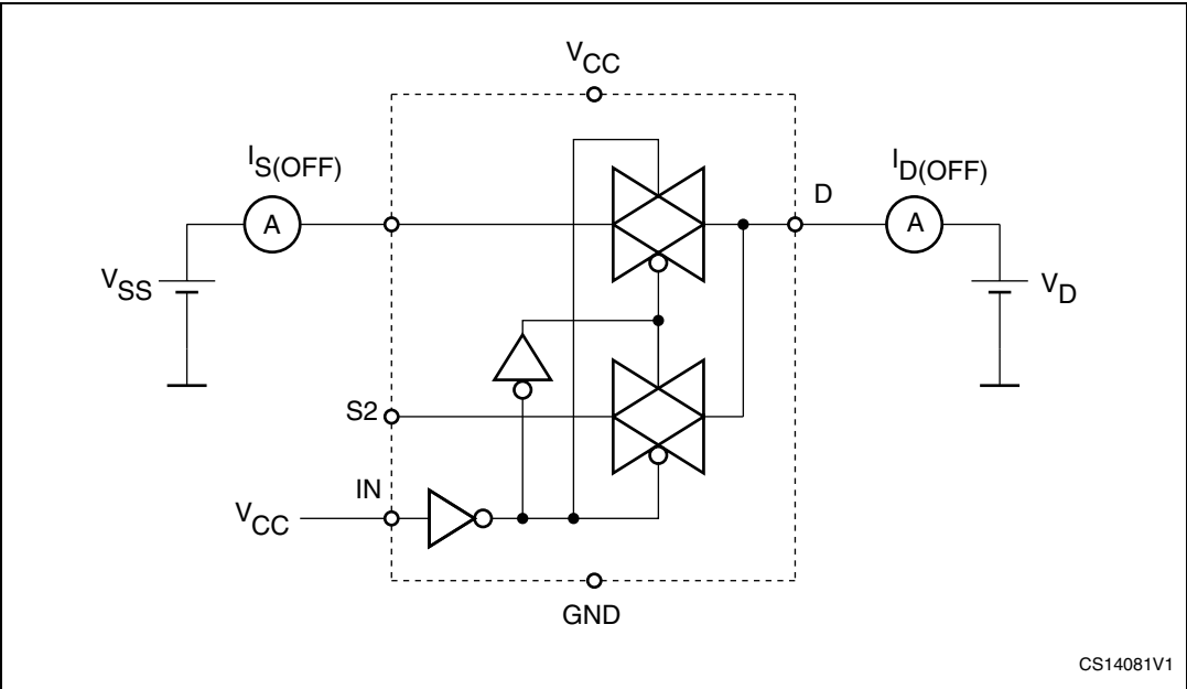
Figure 7. OFF leakage
