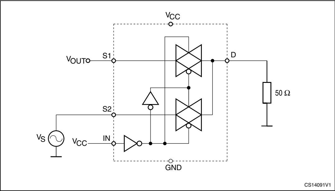
Figure 8. Channel-to-channel crosstalk
