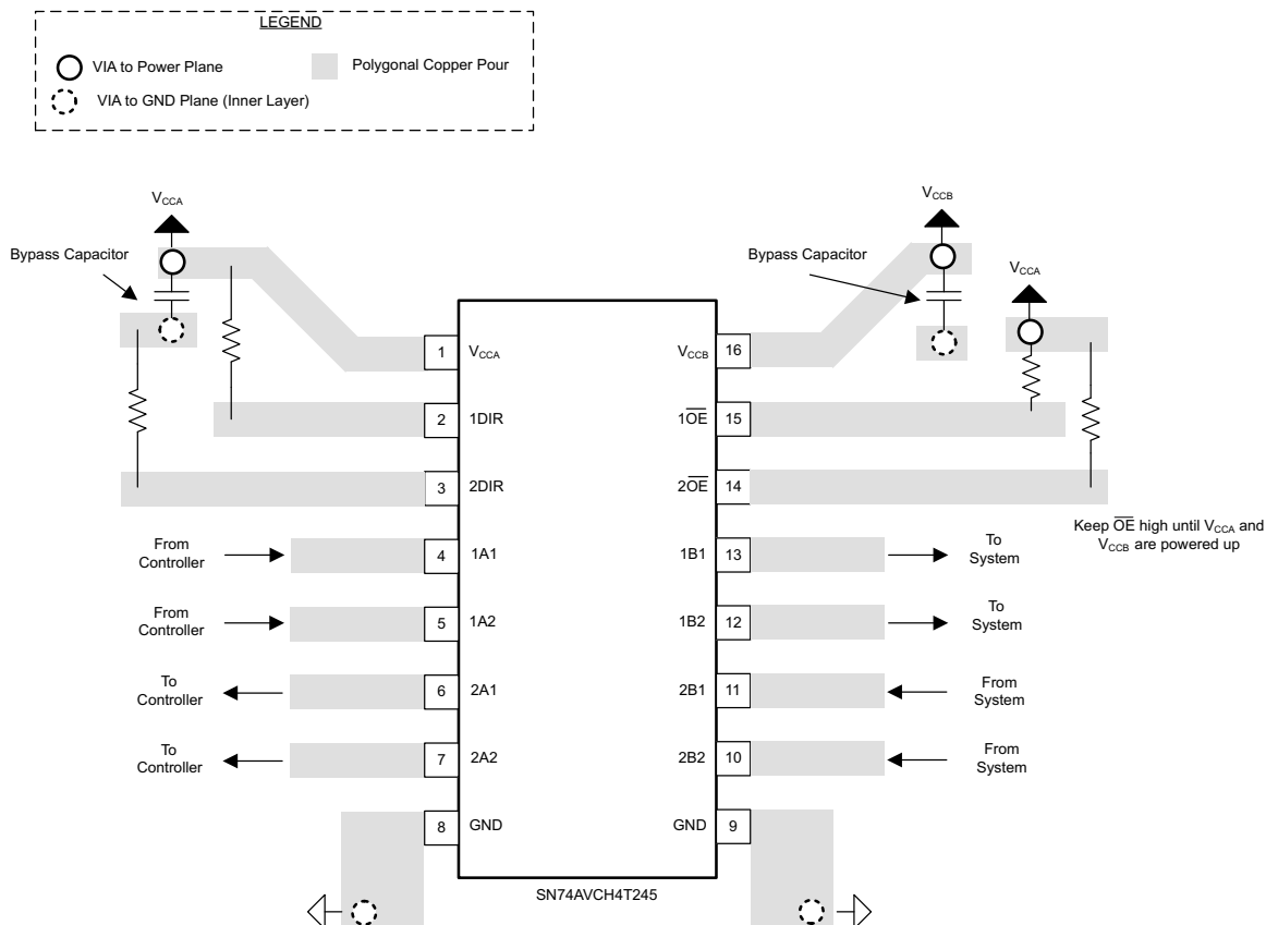
Figure 8-3. Layout Recommendation
