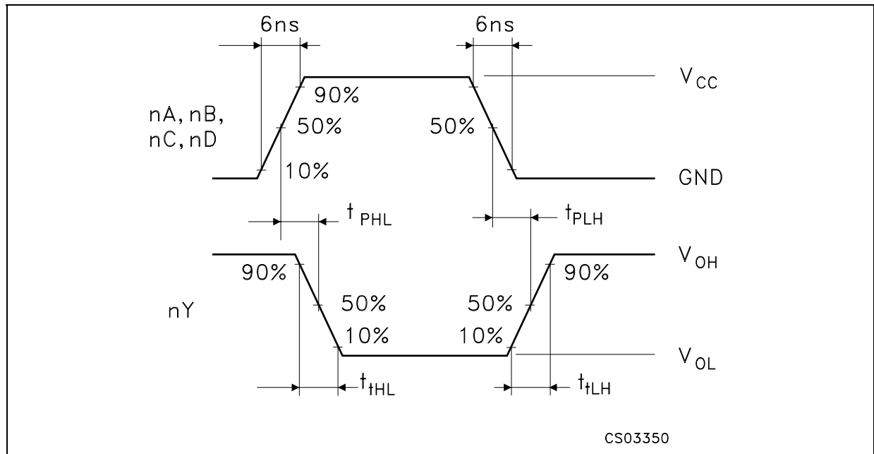
WAVEFORM 1: PROPAGATION DELAY TIME ( f=1\text{MHz} ; 50% duty cycle)
