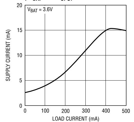
1.5x Mode Supply Current vs I_{CP0} ( I_{VBAT} = 1.5I_{CP0} )
