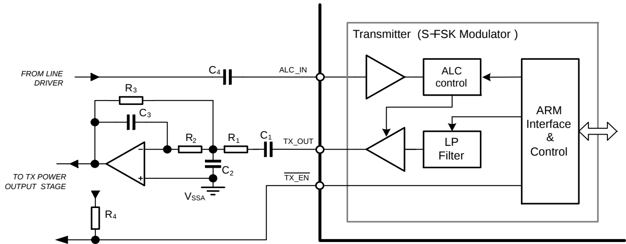
Figure 17. TX_OUT Filter
