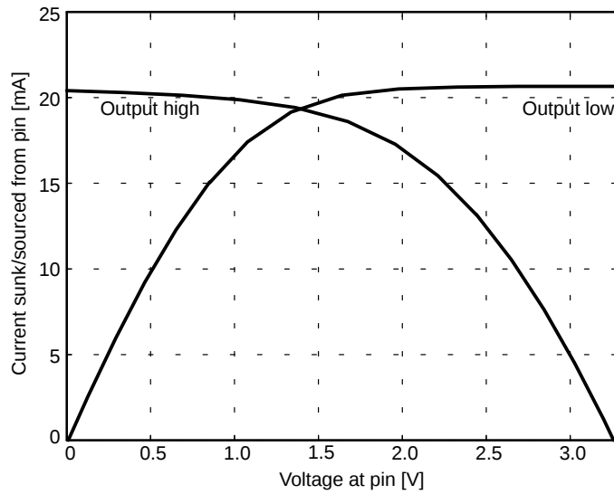
Figure 8. GPIO Current Sourcing and Sinking Capability
