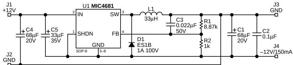
Figure 8. +12V to -12V/150mA Buck-Boost Converter
