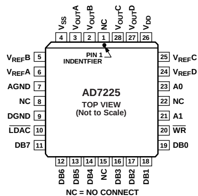
Figure 3. PLCC
