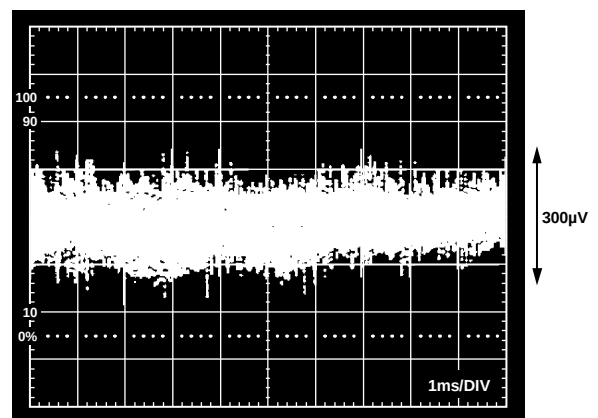
Figure 9. Broadband Noise
