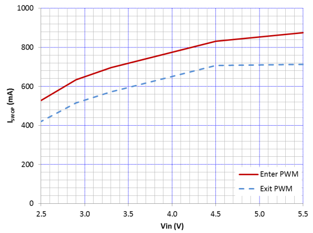
Figure 29. Switchover Point V_{OUT} = 1.4 \text{ V}
