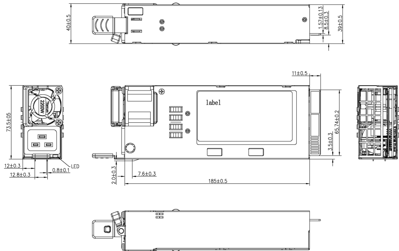
Figure 16. Mechanical Drawing
