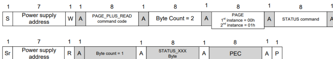
Figure 4. Reading STATUS commands with PAGE_PLUS_READ
