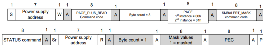
Figure 6. PAGE_PLUS_READ command.
