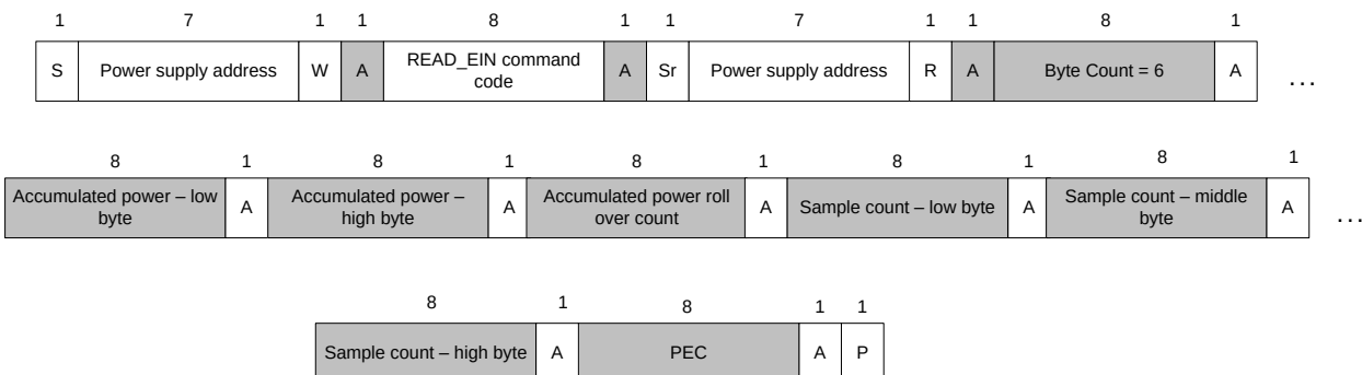
Figure 9. READ_EIN Command
