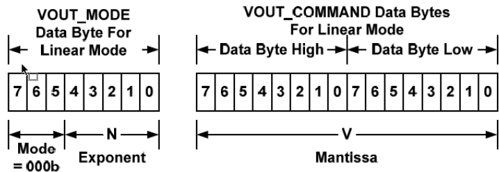
Figure 12. Linear Format Data Bytes
