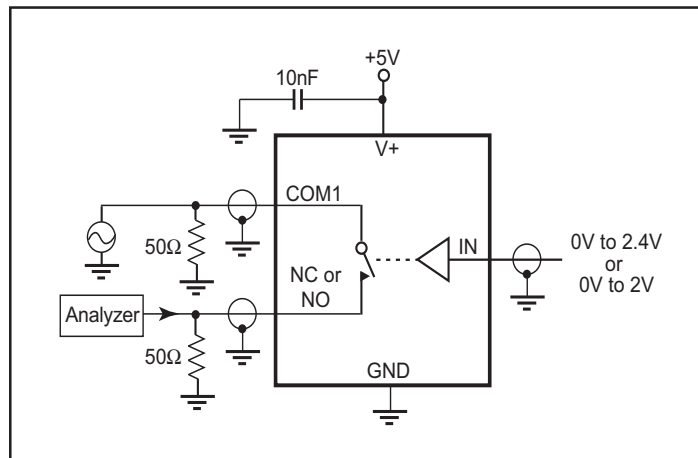
Figure 5. Off Isolation/On-Channel Bandwidth
