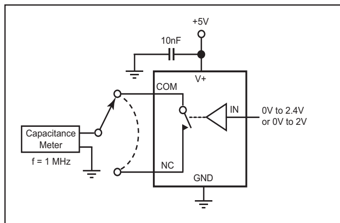
Figure 7. Channel-Off Capacitance
