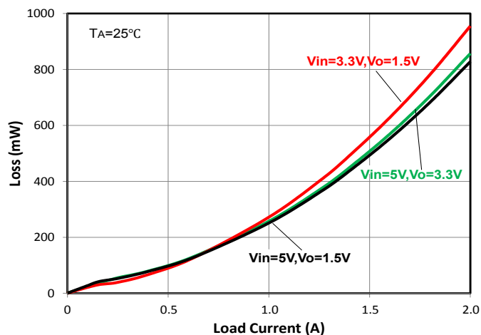
Total Loss (Per Channel) vs. Load Current
