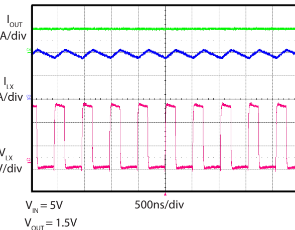
Steady State (PWM) Operation ( I_{OUT} = 2A )
