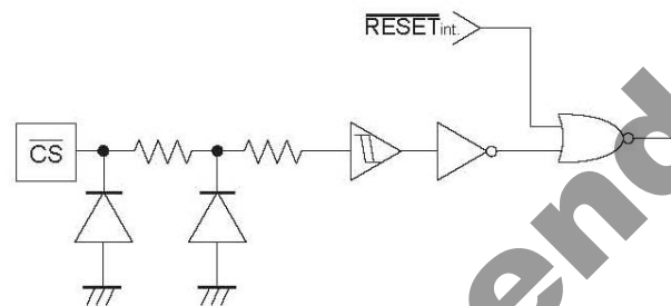
Figure 56. \overline{\text{CS}} input equivalent circuit
