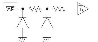
Figure 60. \overline{\text{WP}} input equivalent circuit
