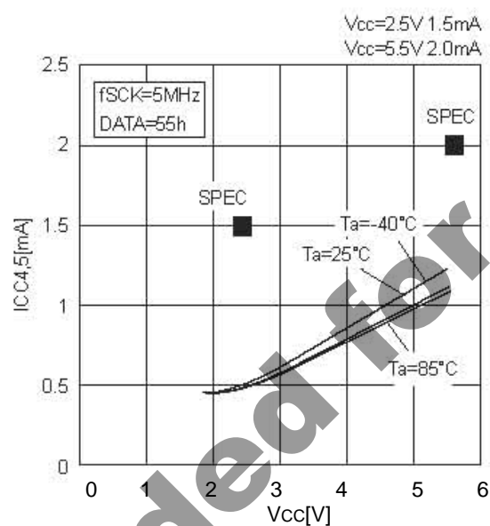
Figure 13. Consumption current at READ operation ICC4,5 (READ, WRSR, fSCK=5MHz)
