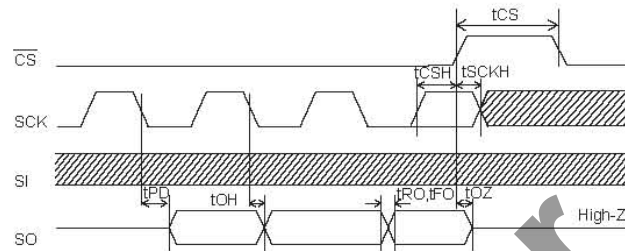
Figure 2. Input / output timing
