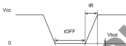
Figure 62. Rise waveform
