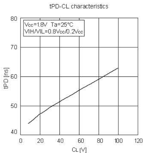
Figure 54. SO load dependency of data output delay time
