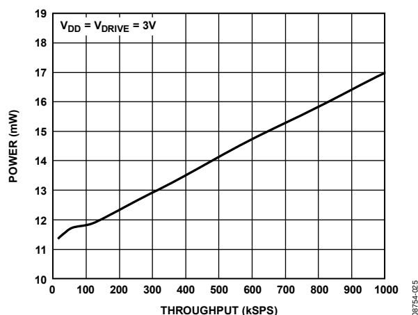
Figure 18. Power vs. Throughput in Normal Mode with V_{DD} = 3\text{ V}
