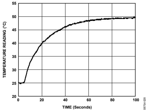
Figure 10. Response to Thermal Shock from Room Temperature into 50°C Stirred Oil
