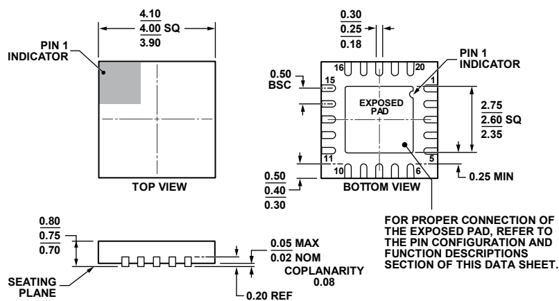
COMPLIANT TO JEDEC STANDARDS MO-220-WGGD. Figure 32. 20-Lead Lead Frame Chip Scale Package [LFCSP_WQ] 4 mm x 4 mm Body, Very, Very Thin Quad (CP-20-8) Dimensions shown in millimeters
