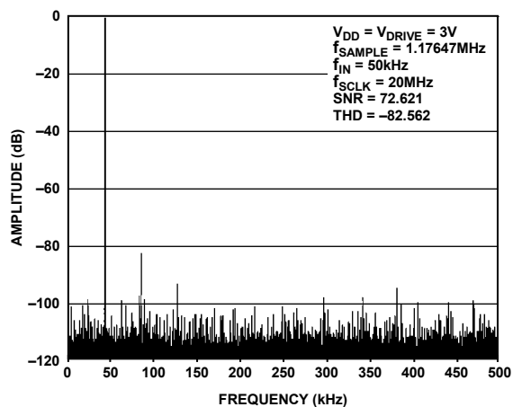
Figure 3. Typical FFT
