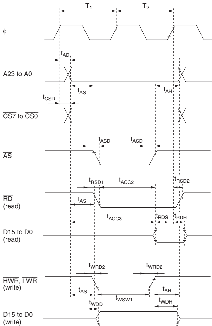
Figure 25.7 Basic Bus Timing (Two-State Access)
