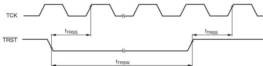
Figure 26.22 Boundary Scan \overline{\text{TRST}} Input Timing (At Reset Hold)
