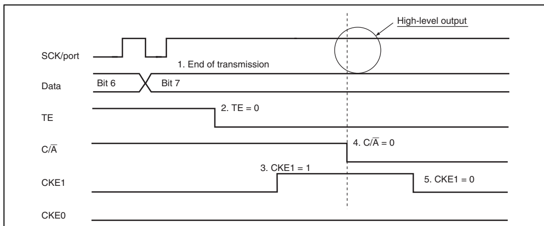
Figure 13.45 Operation when Switching from SCK Pin Function to Port Pin Function (Example of Preventing Low-Level Output)
