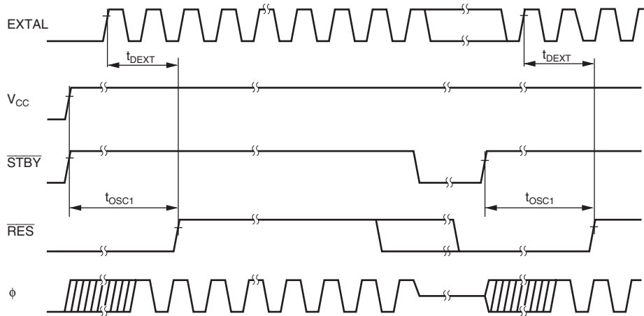
Figure 26.4 Oscillation Stabilization Timing
