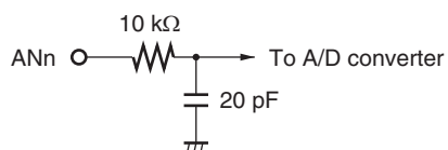
Figure 16.11 Analog Input Pin Equivalent Circuit
