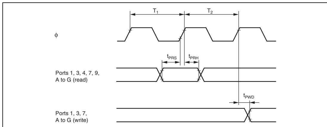
Figure 26.12 I/O Port Input/Output Timing
