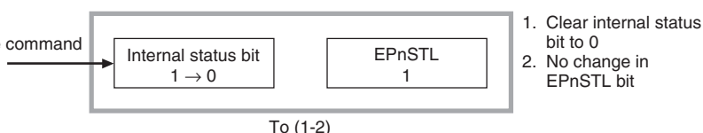
Figure 15.23 Forcible Stall by Firmware
