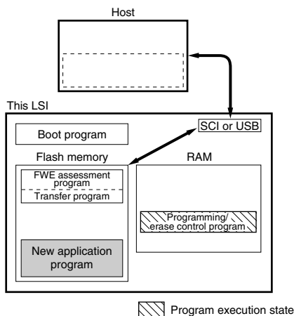
Figure 19.4 User Program Mode (Sample)
