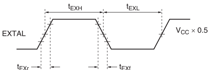
Figure 21.6 External Clock Input Timing
