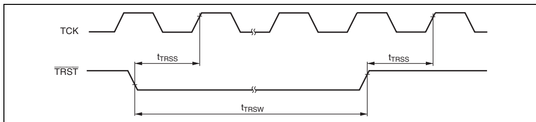
Figure 24.22 Boundary Scan \overline{TRST} Input Timing (At Reset Hold)
