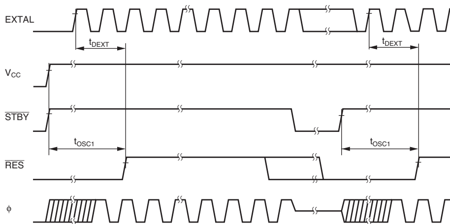
Figure 24.4 Oscillation Stabilization Timing
