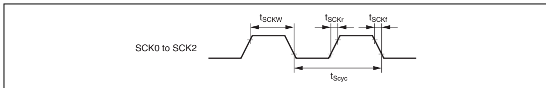
Figure 26.18 SCK Clock Input Timing
