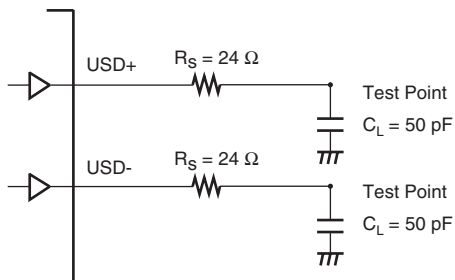
Figure 27.25 Test Load Circuit
