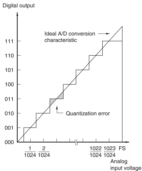
Figure 16.7 A/D Conversion Precision Definitions (1)
