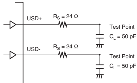
Figure 25.25 Test Load Circuit
