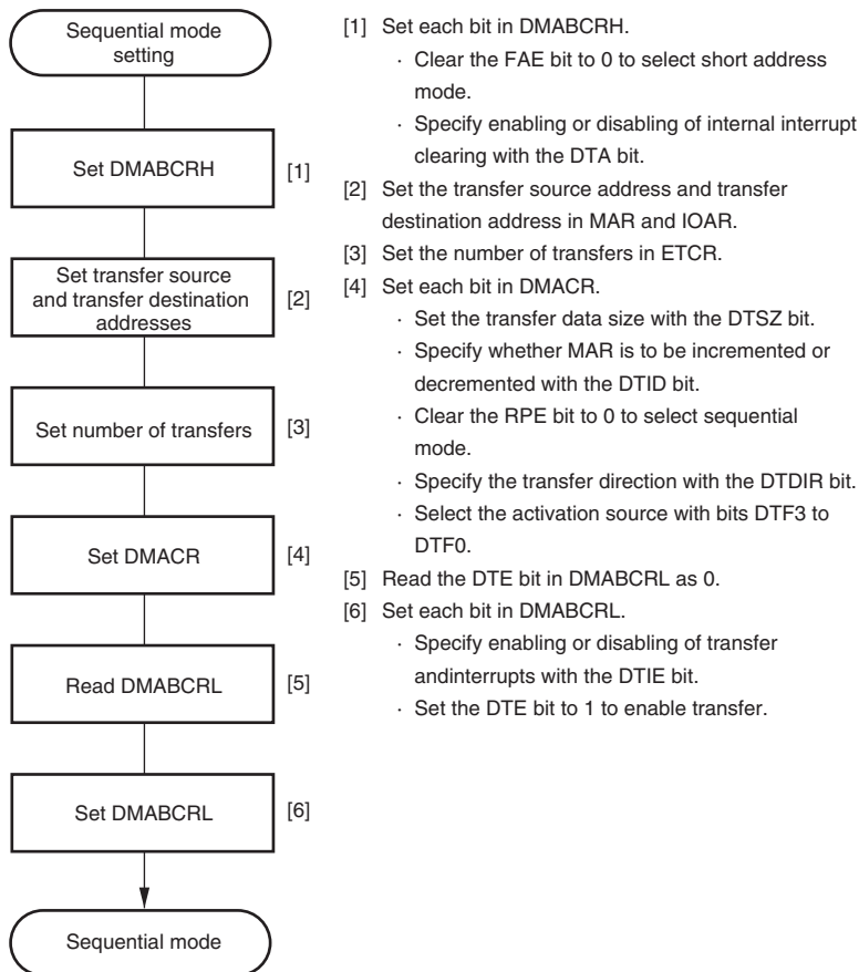
Figure 7.4 Example of Sequential Mode Setting Procedure
