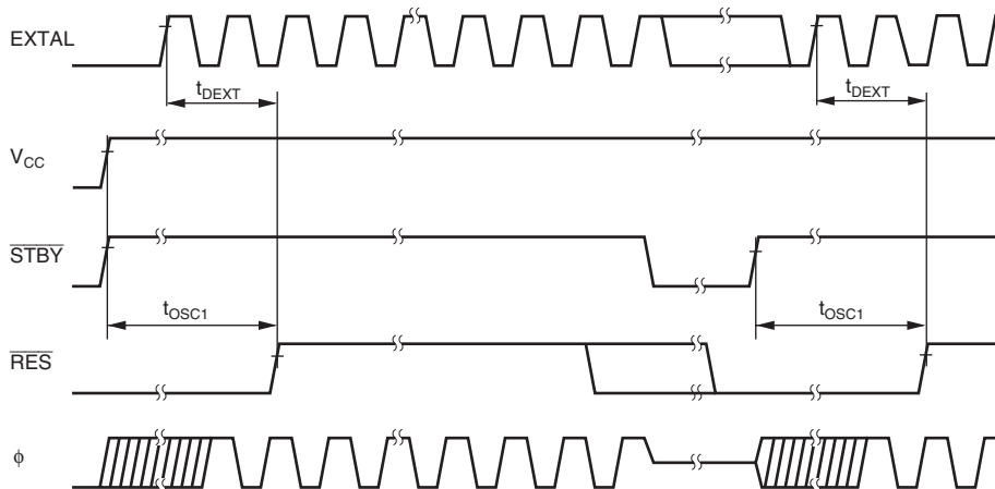
Figure 25.4 Oscillation Stabilization Timing
