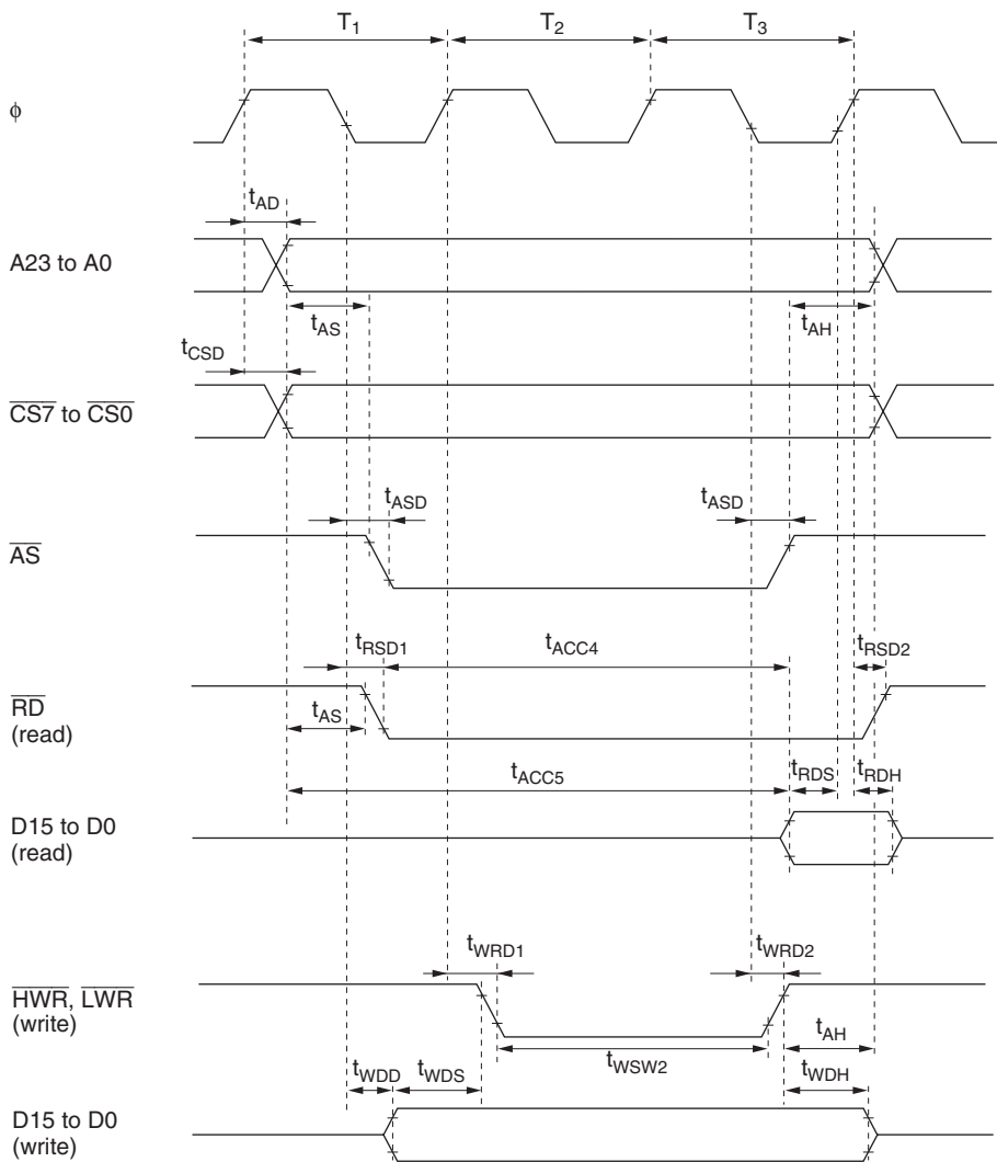
Figure 24.8 Basic Bus Timing (Three-State Access)
