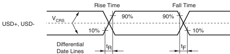
Figure 27.24 Data Signal Timing
