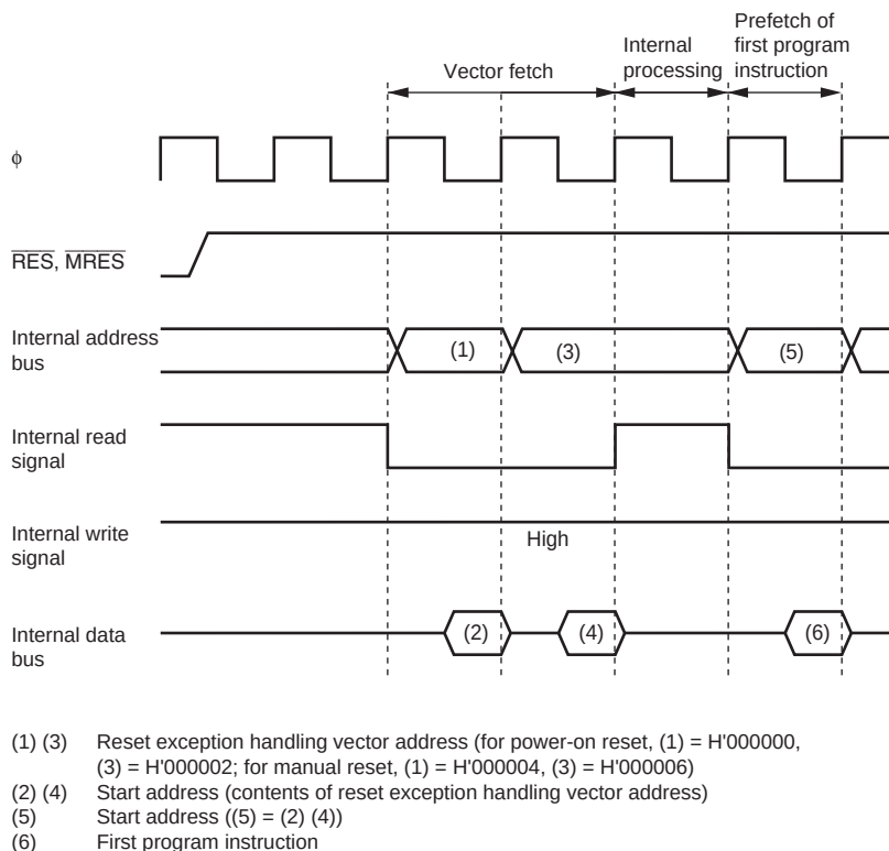
Figure 4.2 Reset Sequence (Modes 6, 7)
