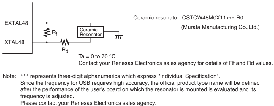
Figure 21.7 Connection of Ceramic Resonator
