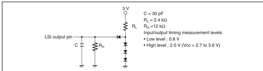
Figure 27.2 Output Load Circuit
