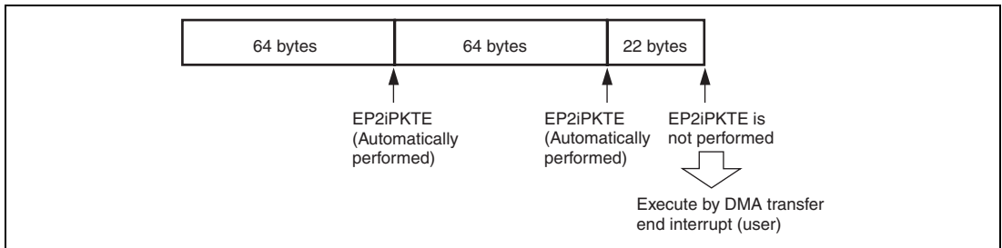
Figure 15.25 EP2iPKTE Operation in UTRG0
