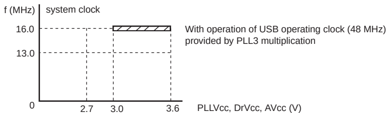
Figure 24.1 Power Supply Voltage and Operating Ranges
