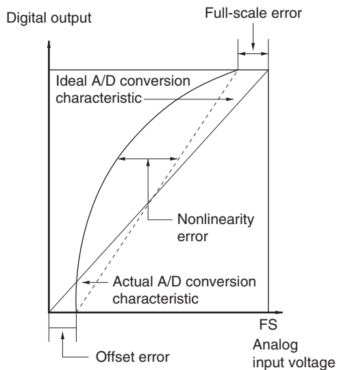
Figure 16.8 A/D Conversion Precision Definitions (2)
