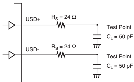
Figure 24.25 Test Load Circuit
