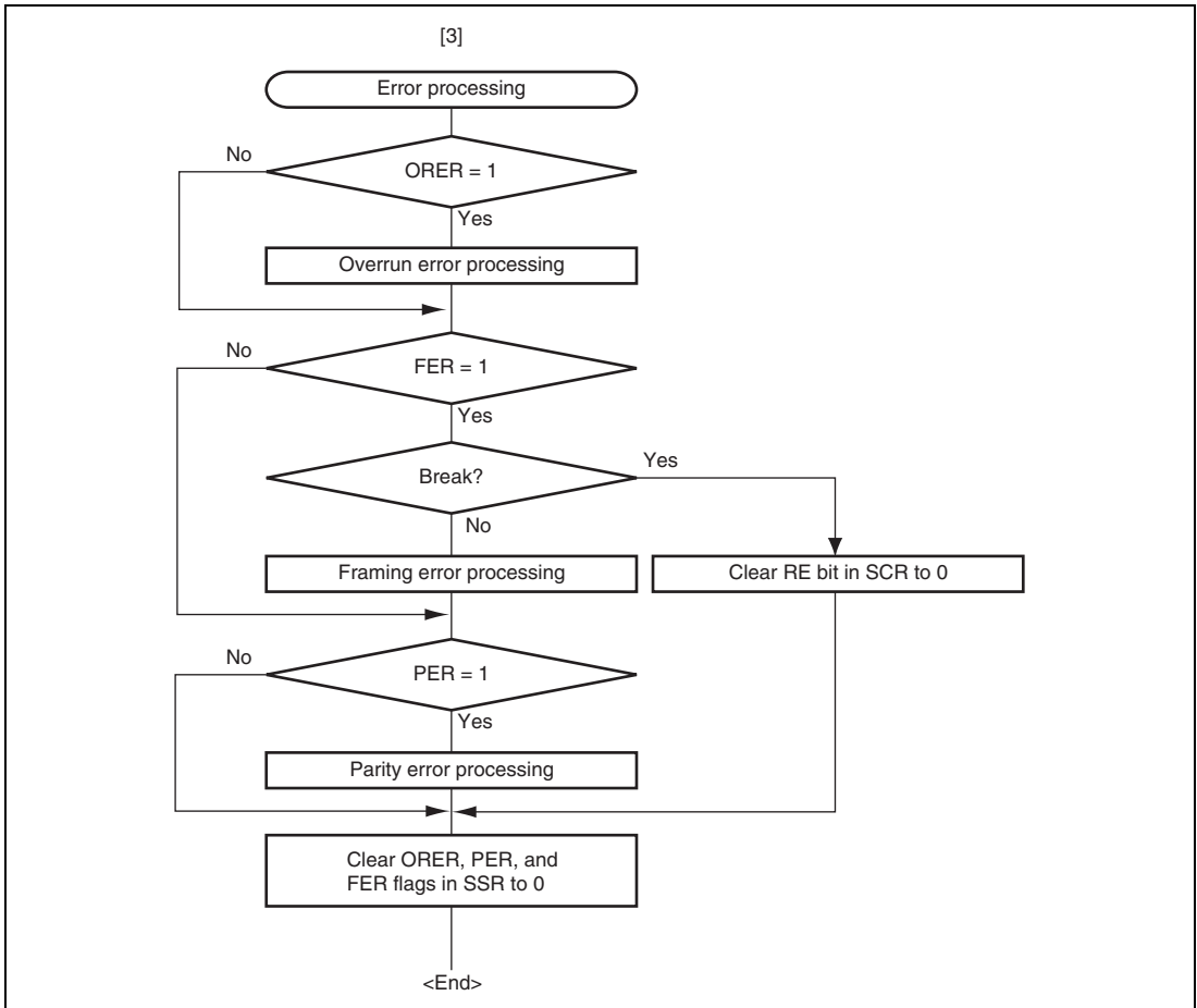
Figure 13.13 Sample Serial Reception Data Flowchart (2)
