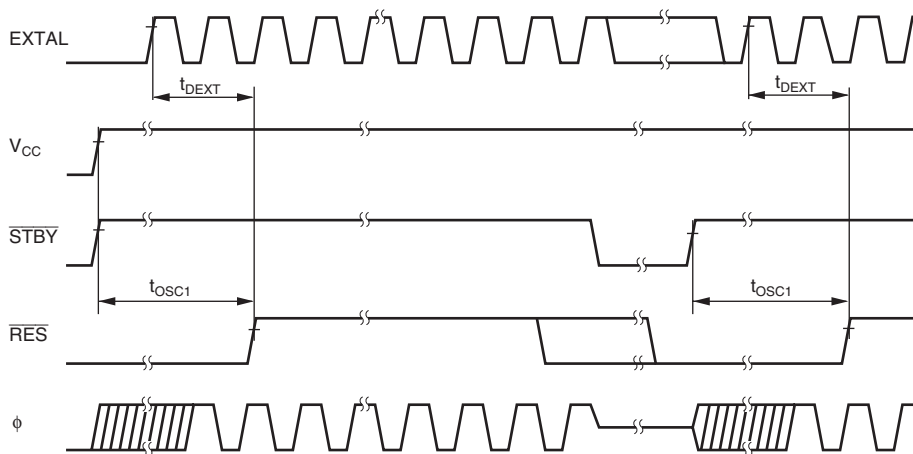
Figure 27.4 Oscillation Stabilization Timing
