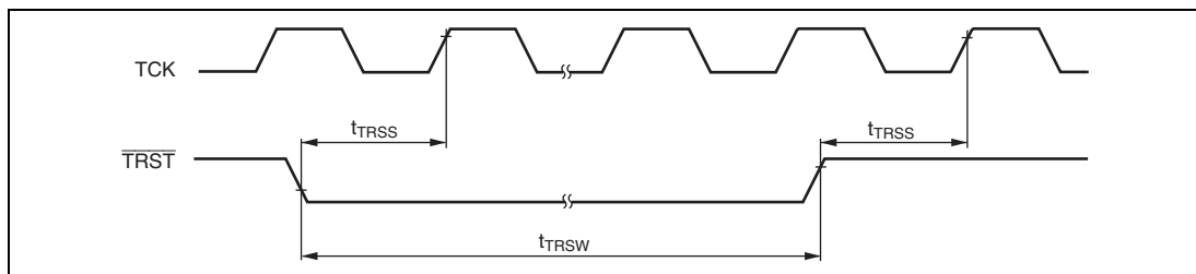
Figure 25.22 Boundary Scan \overline{TRST} Input Timing (At Reset Hold)
