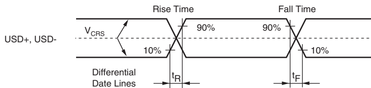
Figure 24.24 Data Signal Timing
