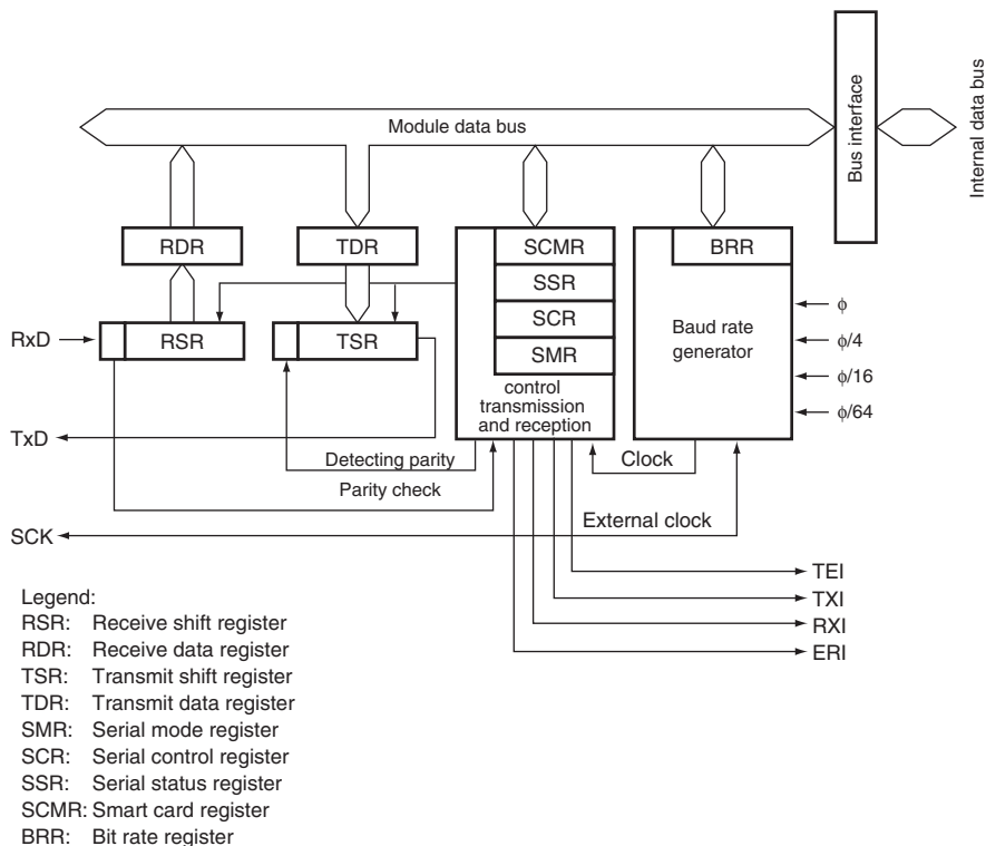
Figure 13.3 Block Diagram of SCI_1 and SCI_2
