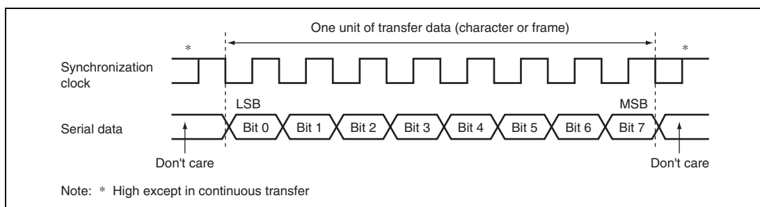
Figure 13.18 Data Format in Synchronous Communication (For LSB-First)
