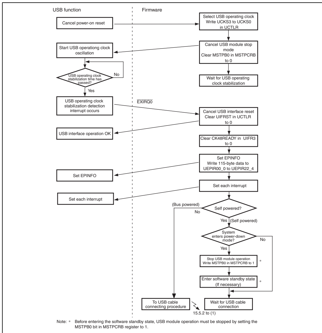
Figure 15.3 USB Initialization
