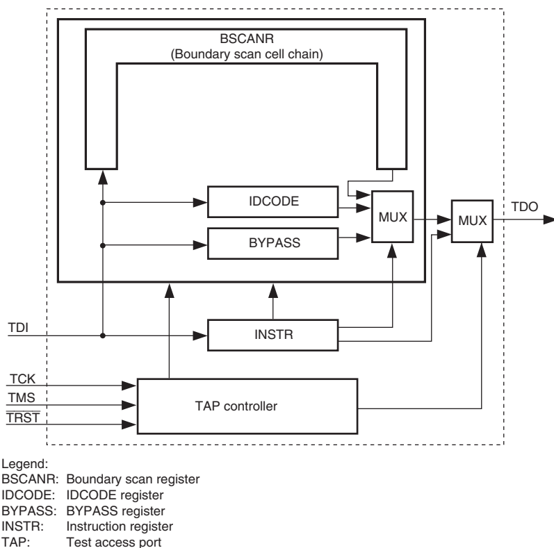
Figure 14.1 Block Diagram of Boundary Scan Function
