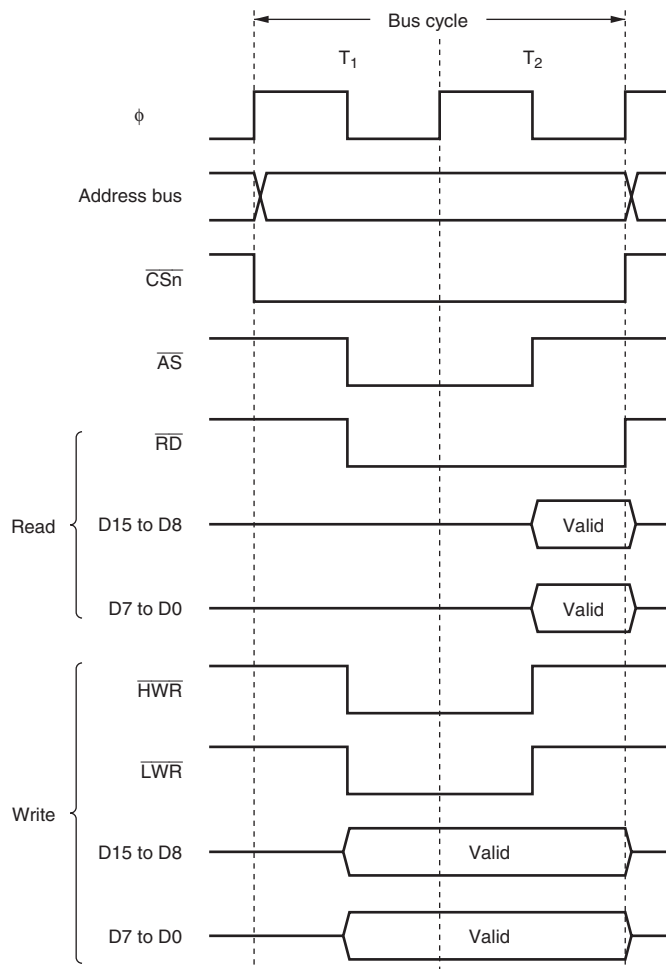
Figure 6.15 Bus Timing for 16-Bit 2-State Access Space (3) (Word Access)
