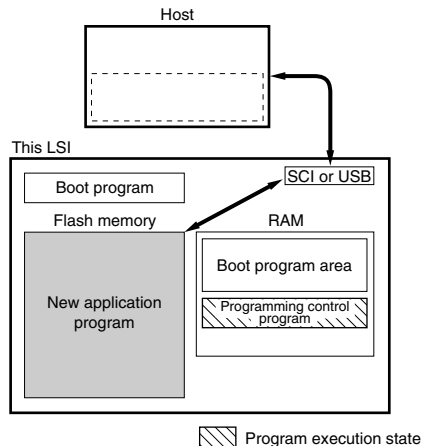
Figure 19.3 Boot Mode (Sample)
