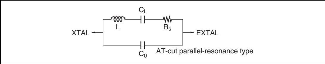
Figure 21.3 Crystal Resonator Equivalent Circuit
