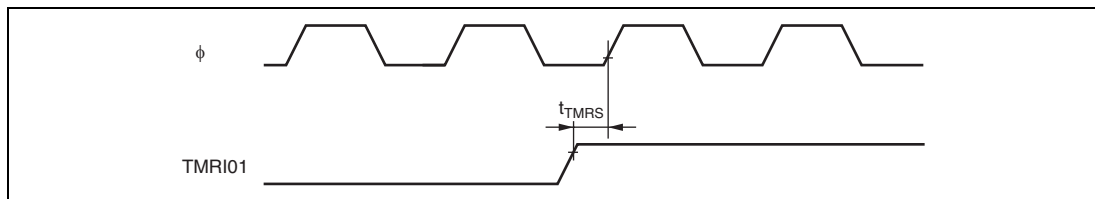
Figure 26.17 8-bit Timer Reset Input Timing
