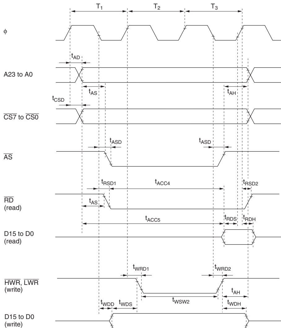
Figure 25.8 Basic Bus Timing (Three-State Access)
