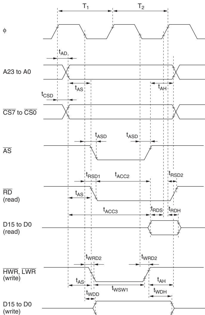
Figure 26.7 Basic Bus Timing (Two-State Access)
