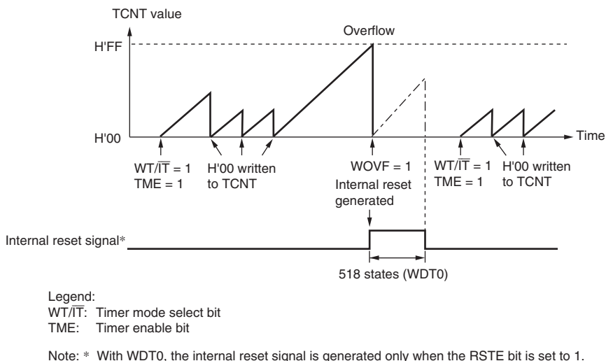
Figure 12.2 Operation in Watchdog Timer Mode
