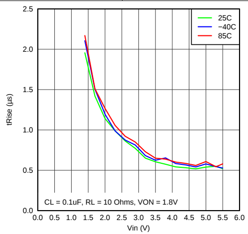
Figure 19. Rise Time vs Input Voltage
