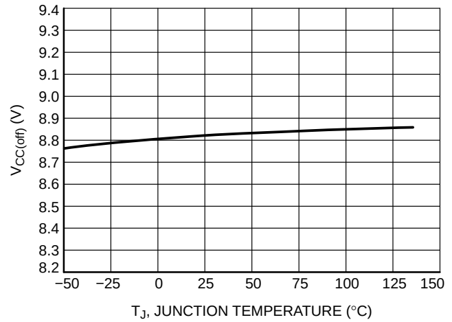
Figure 4. V CC Minimum Operating Voltage vs. Temperature
