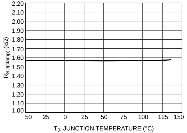
Figure 44. SD Pin Clamp Series Resistor vs. Temperature
