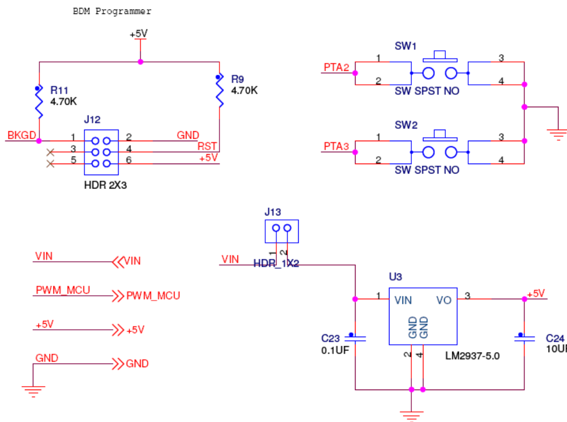
Figure 5. EVB Schematic (3)
