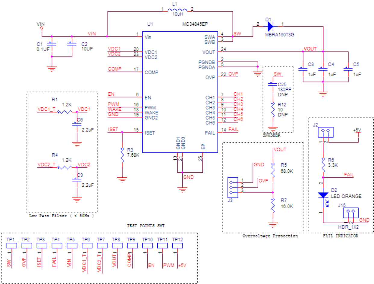
Figure 3. EVB Schematic (1)
