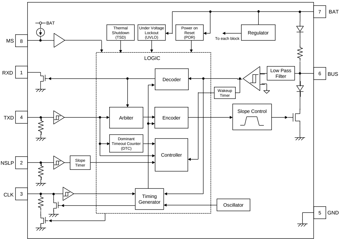
Figure 3. Block Diagram
