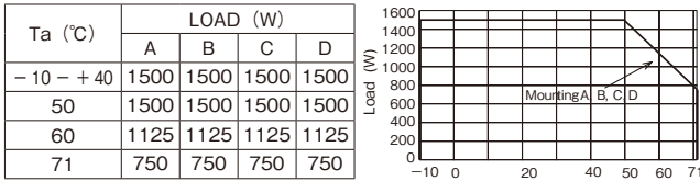
HWS1800T 6V-15V Output Derating
