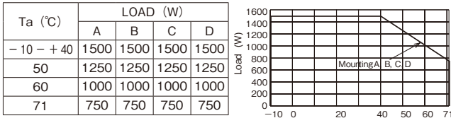
HWS1800T 5V Output Derating
