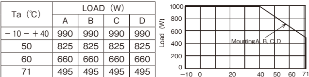
HWS1800T 3V Output Derating
