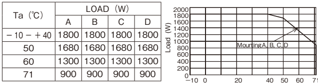
HWS1800T 24V-60V Output Derating
