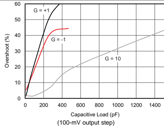
Figure 28. Small-Signal Overshoot vs Capacitive Load
