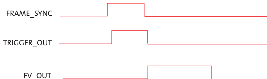
Figure 10: Single-Shot Mode
