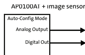
Figure 41: Auto-Config Mode
