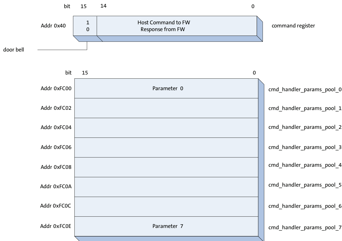
Figure 40: Interface Structure
