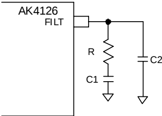
Figure 3. AK4126
