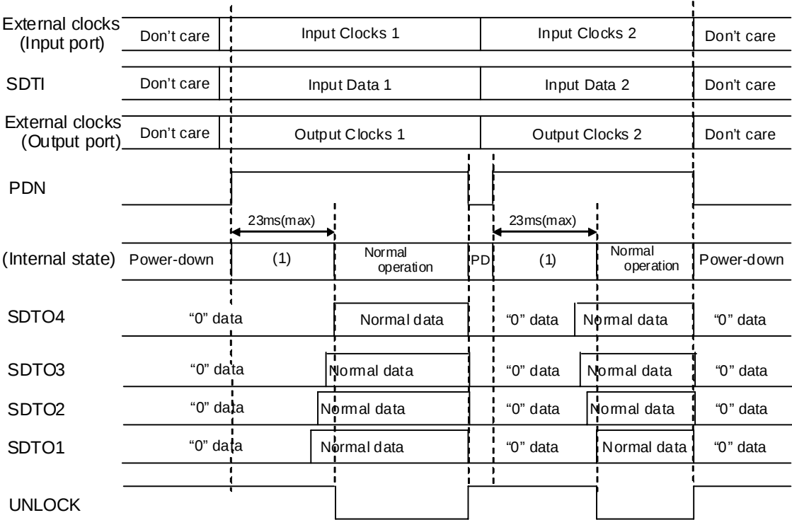
Case 1: System Reset with clock inputs
