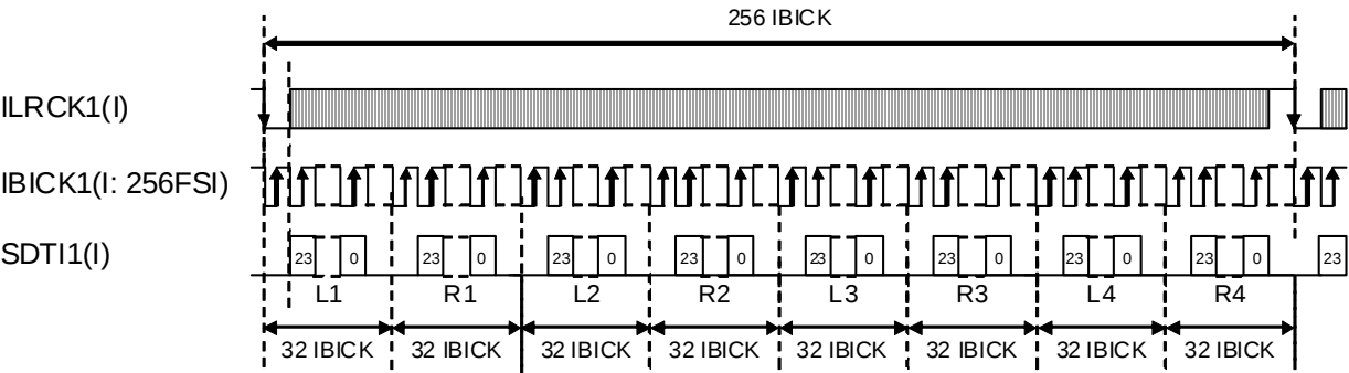
Figure 20. Mode 6 Timing (TDM, I²S, SDTI2-4: Don't care)
