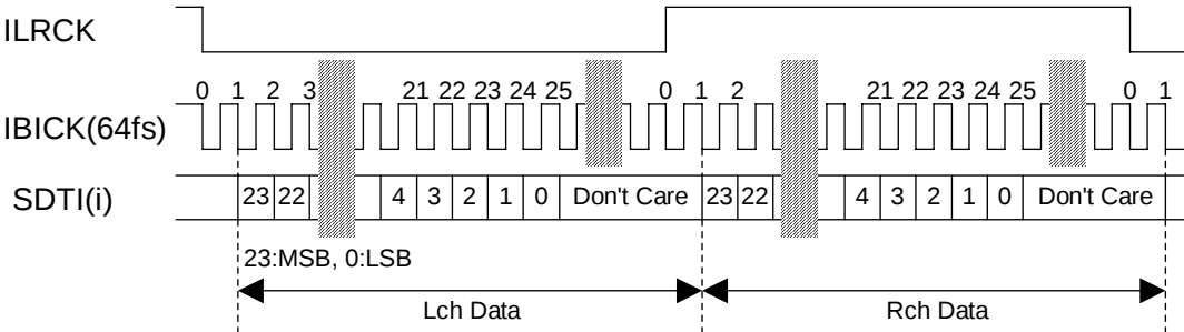
Figure 17. Mode 3 Timing (24bit I²S)
