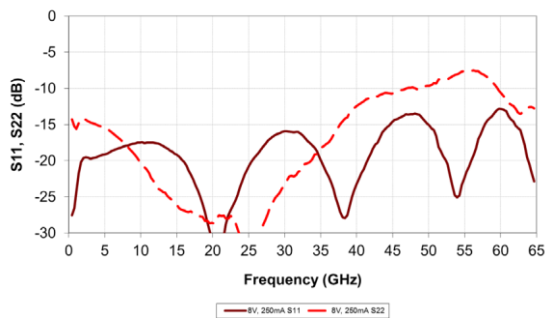
S11, S22
