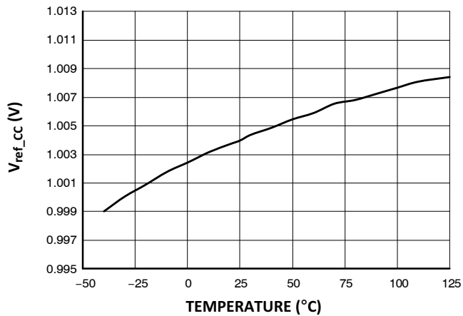
Figure 13. V_{ref\_CC} vs. Junction Temperature
