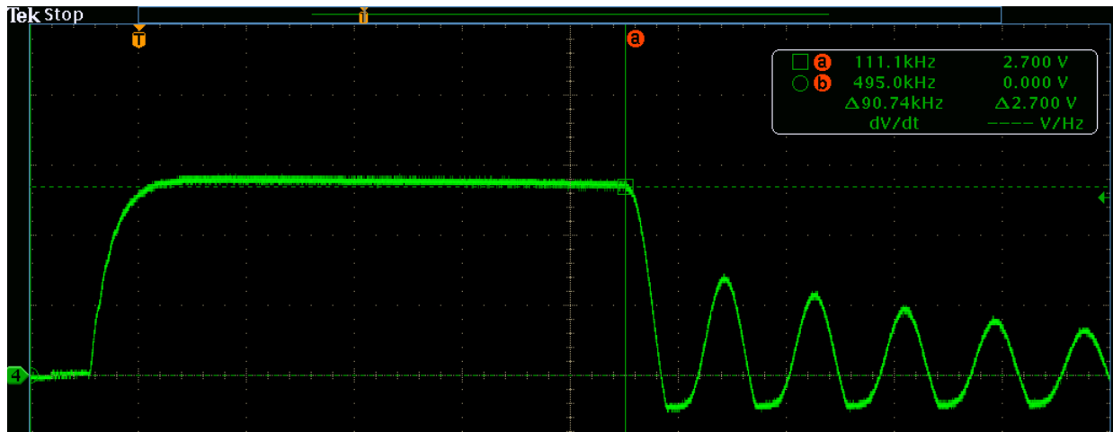
Figure 31. ZCD Voltage Waveform during Constant Voltage Regulation
