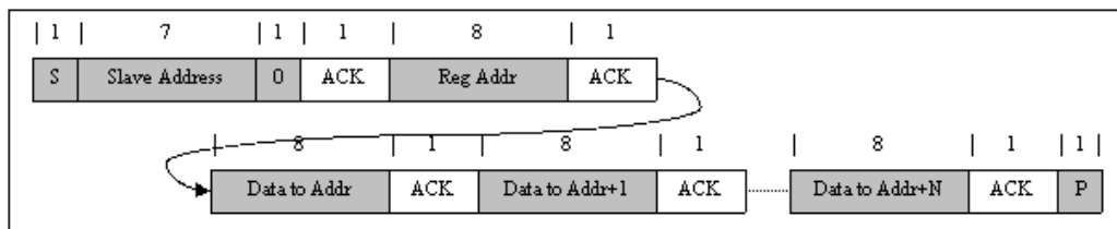
Figure 14. Multi Write
