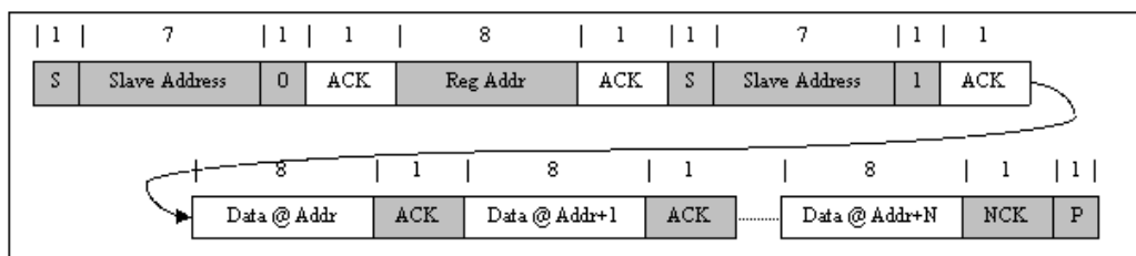
Figure 15. Multi Read
