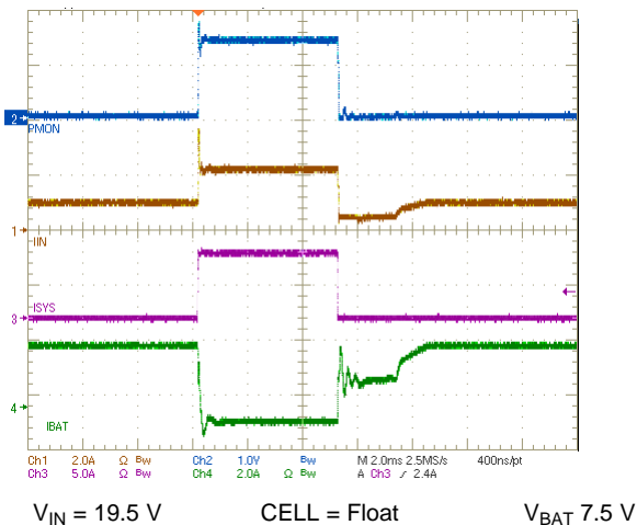
Figure 32. Transient Response, Charge Disabled, In Supplement Mode
