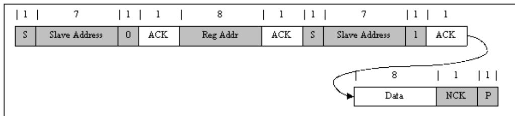
Figure 13. Single Read
