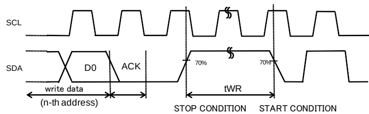
Figure 2-(c). Write Cycle Timing
