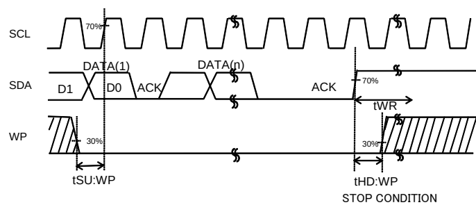
Figure 2-(d). WP Timing at Write Execution
