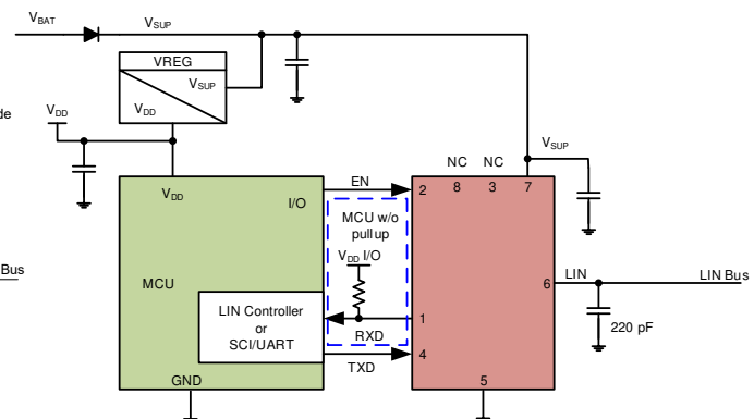
Simplified Schematics, Responder Mode
