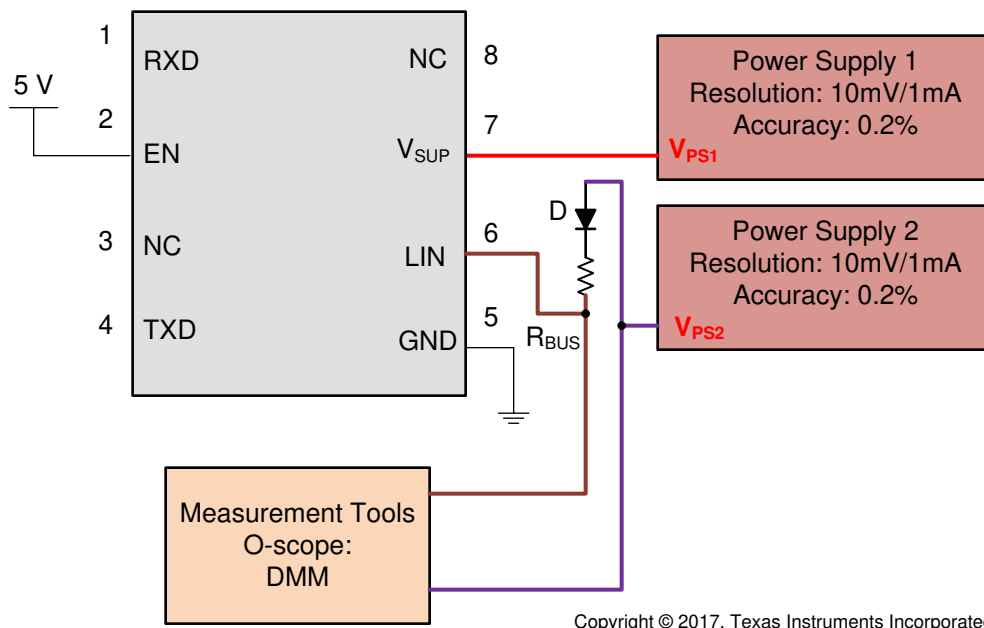
Figure 8-5. V<sub>SUP</sub>_NON_OP Param 11
