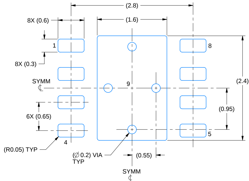
LAND PATTERN EXAMPLE EXPOSED METAL SHOWN SCALE:20X
