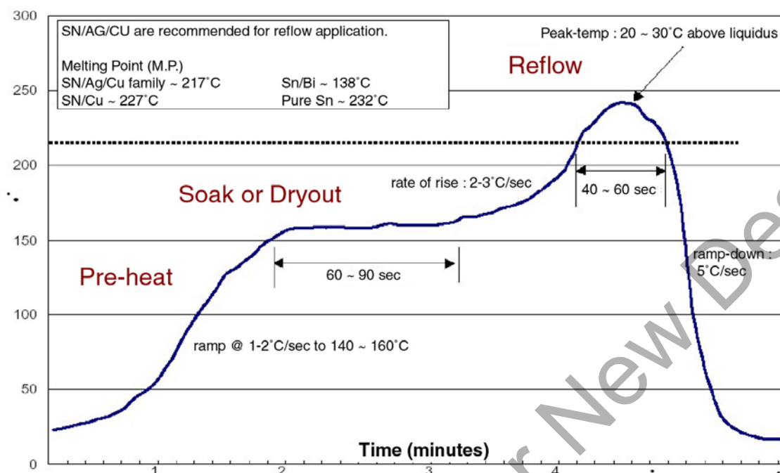
Figure 9.3: Typical reflow profile
