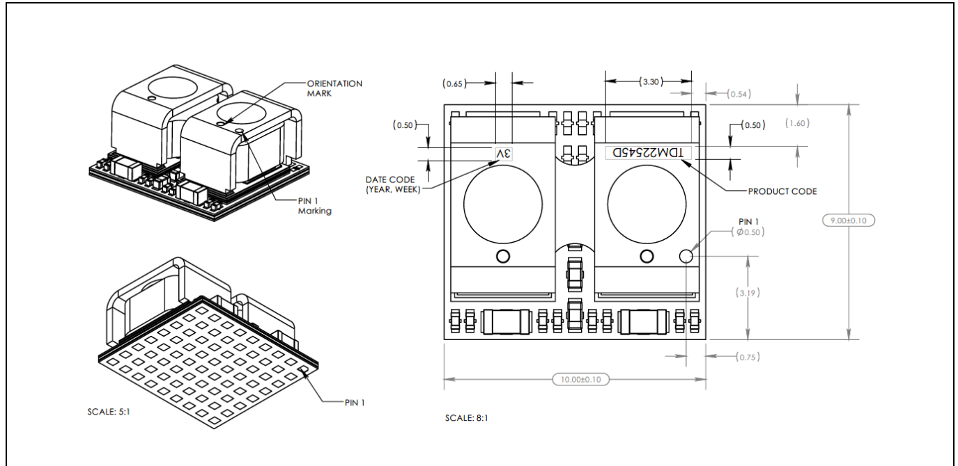
Figure 3 Package Marking
