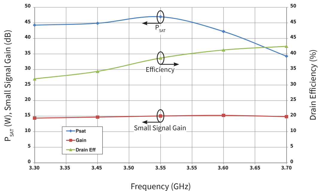
P_{SAT} Small Signal Gain and Drain Efficiency vs Frequency of the CGH40035F in the CGH40035F-AMP
