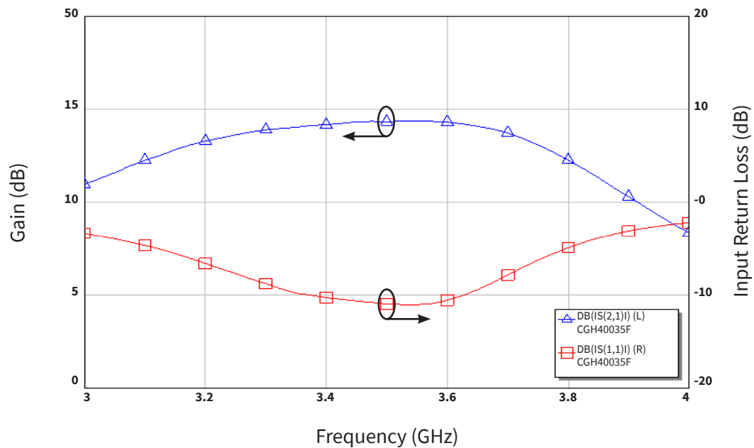
Simulated Small Signal Gain and Input Return Loss of the CGH40035F-AMP vs Frequency
