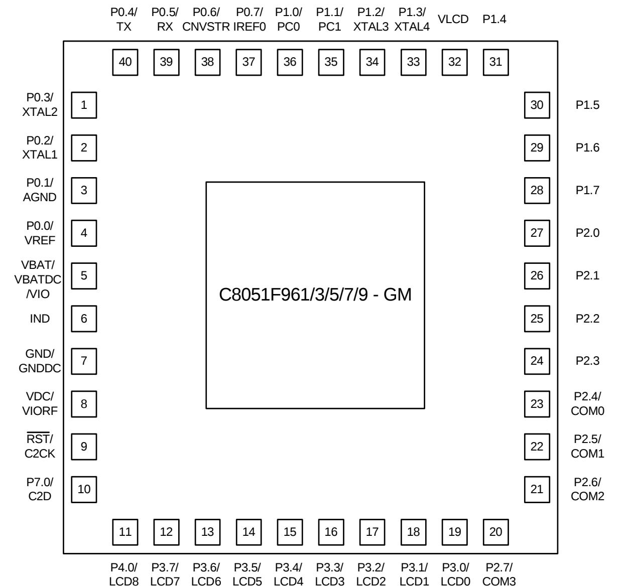
Figure 3.2. QFN-40 Pinout Diagram (Top View)
