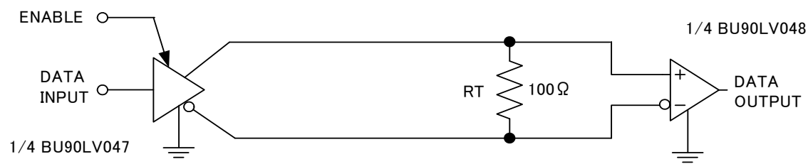
Fig.8. Point-to-Point Application
