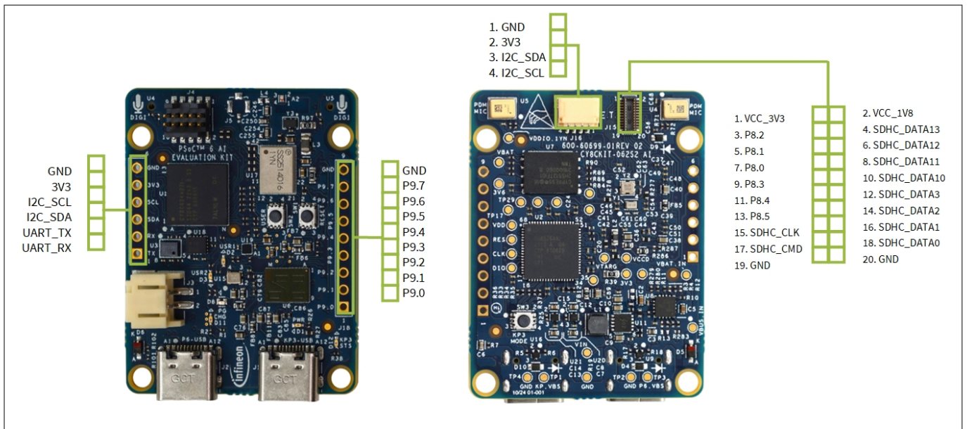
Figure 2 Board pinout
