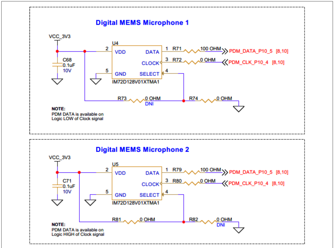
Figure 32 Schematic of digital microphones interface
