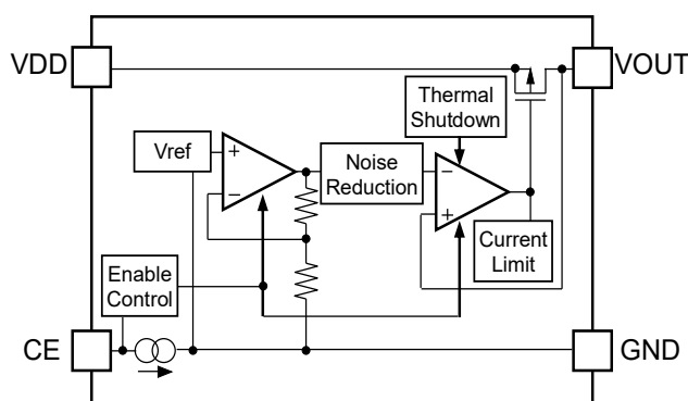
RP123xxxxB Block Diagram
