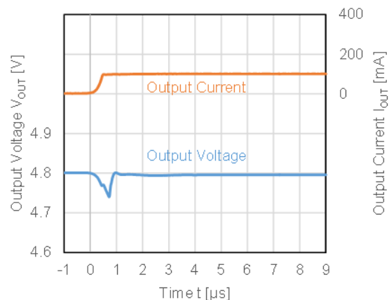
RP123x48xx, V_{IN} = 5.5\text{ V} , I_{OUT} = 0 \Rightarrow 100\text{ mA} , t_R = 0.5\text{ }\mu\text{s}
