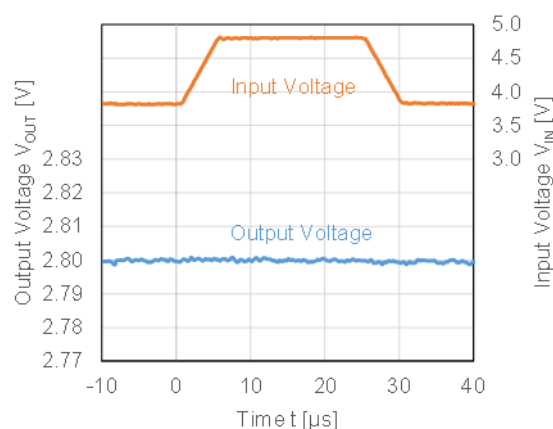
RP123x48xx, I_{OUT} = 20 \text{ mA}
