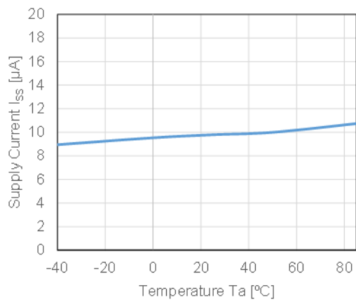
RP123x48xx, V_{IN} = 5.5\text{ V}
