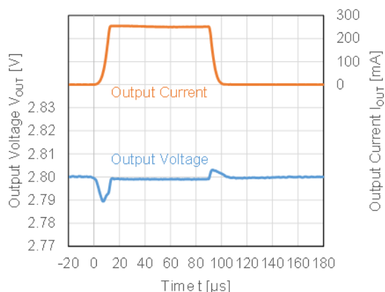
RP123x48xx, V_{IN} = 5.5\text{ V} , I_{OUT} = 1\text{ mA} \Leftrightarrow 250\text{ mA} , t_R = t_F = 10\text{ }\mu\text{s}
