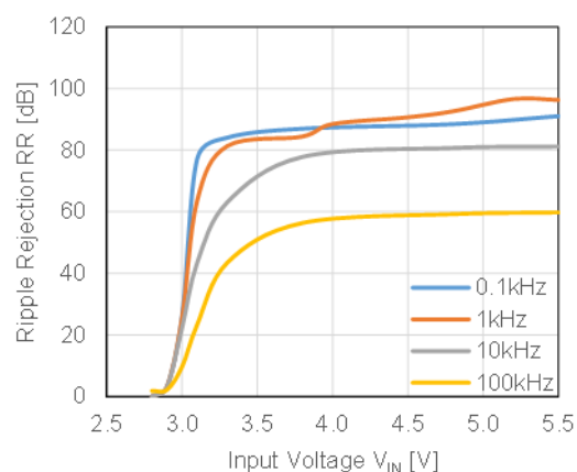
RP123x48xx, I_{OUT} = 250\text{ mA}
