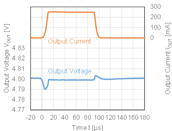
RP123x48xx, V_{IN} = 5.5\text{ V} , I_{OUT} = 1\text{ mA} \Leftrightarrow 250\text{ mA} , t_R = t_F = 10\text{ }\mu\text{s}
