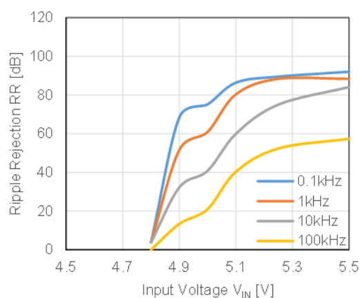
RP123x48xx, I_{OUT} = 100\text{ mA}
