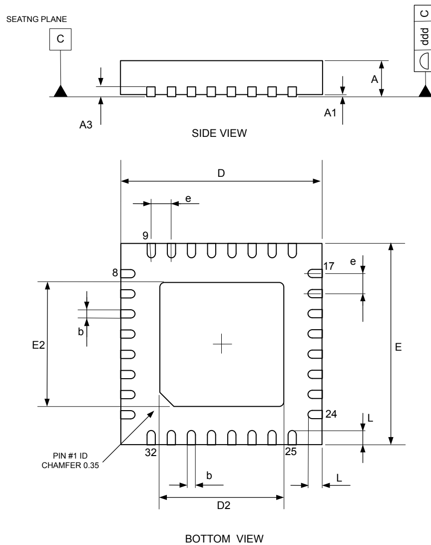
Figure 22. VFQFPN32 - Outline
