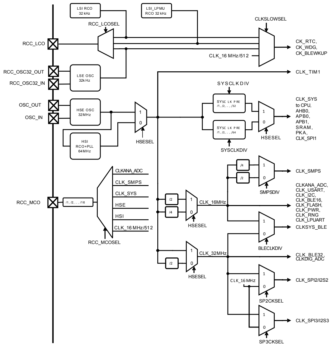
Figure 6. Clock tree
