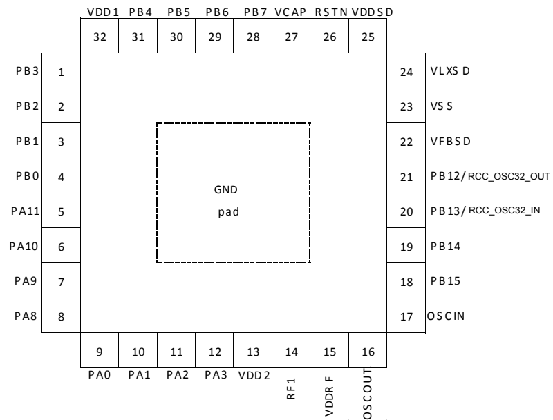
Figure 8. Pinout top view (QFN32 package)
