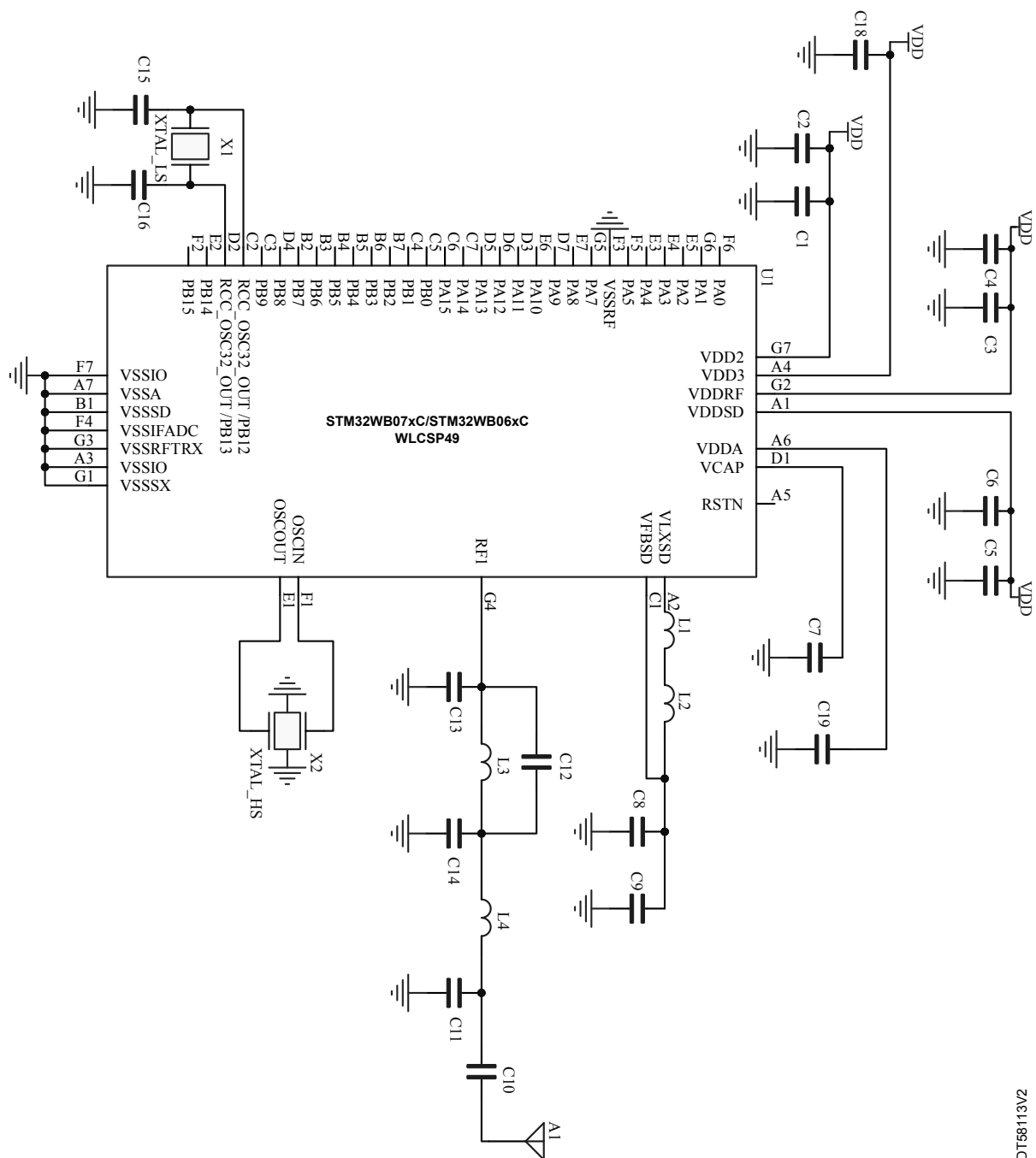
Figure 12. Application circuit: DC-DC converter, WCSP49 package
