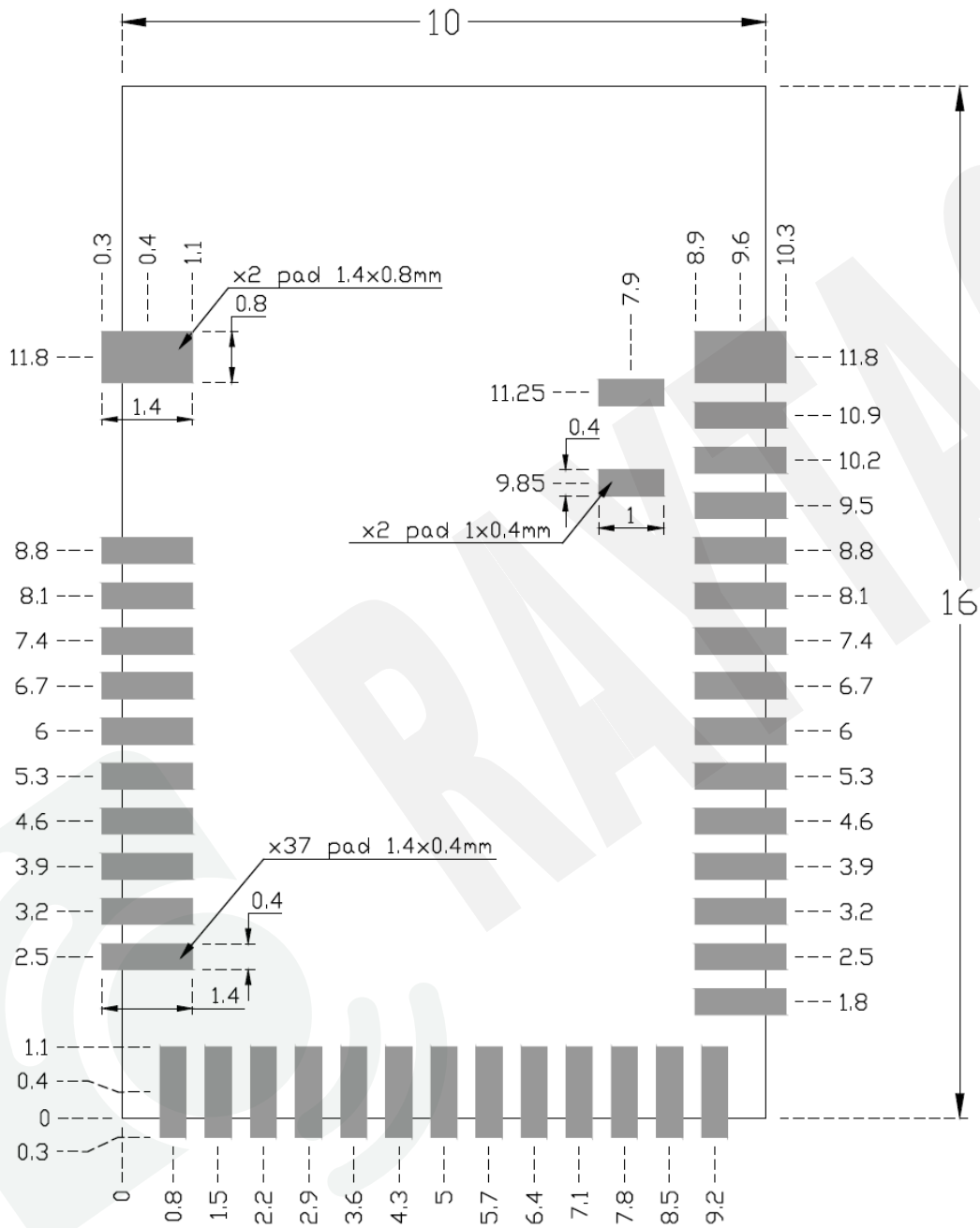
Top View (Unit: mm)
