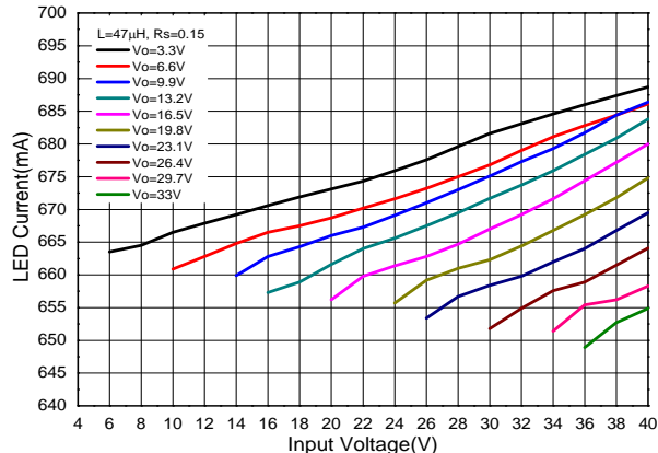
LED Current vs. Input Voltage (TSOT25, R s =0.15Ω, L=47μH)
