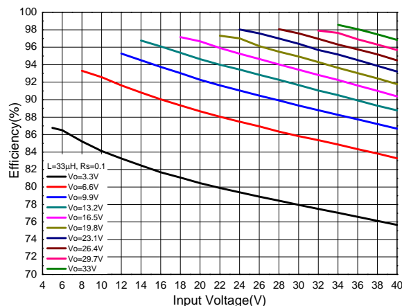
Efficiency vs. Input Voltage (TSOT25, R s =0.1Ω, L=33μH)
