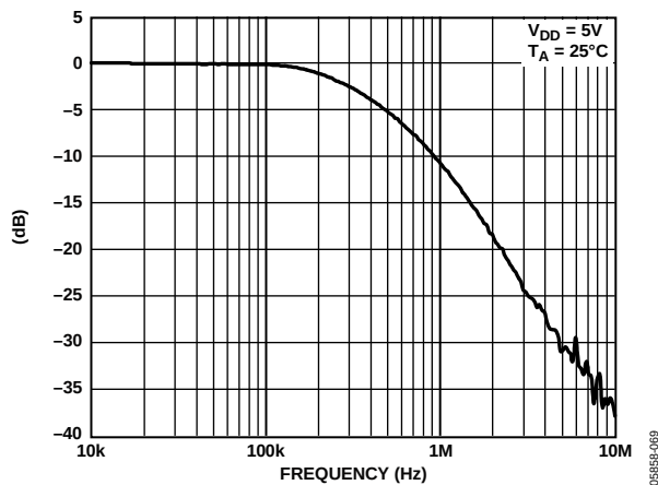
Figure 47. Multiplying Bandwidth
