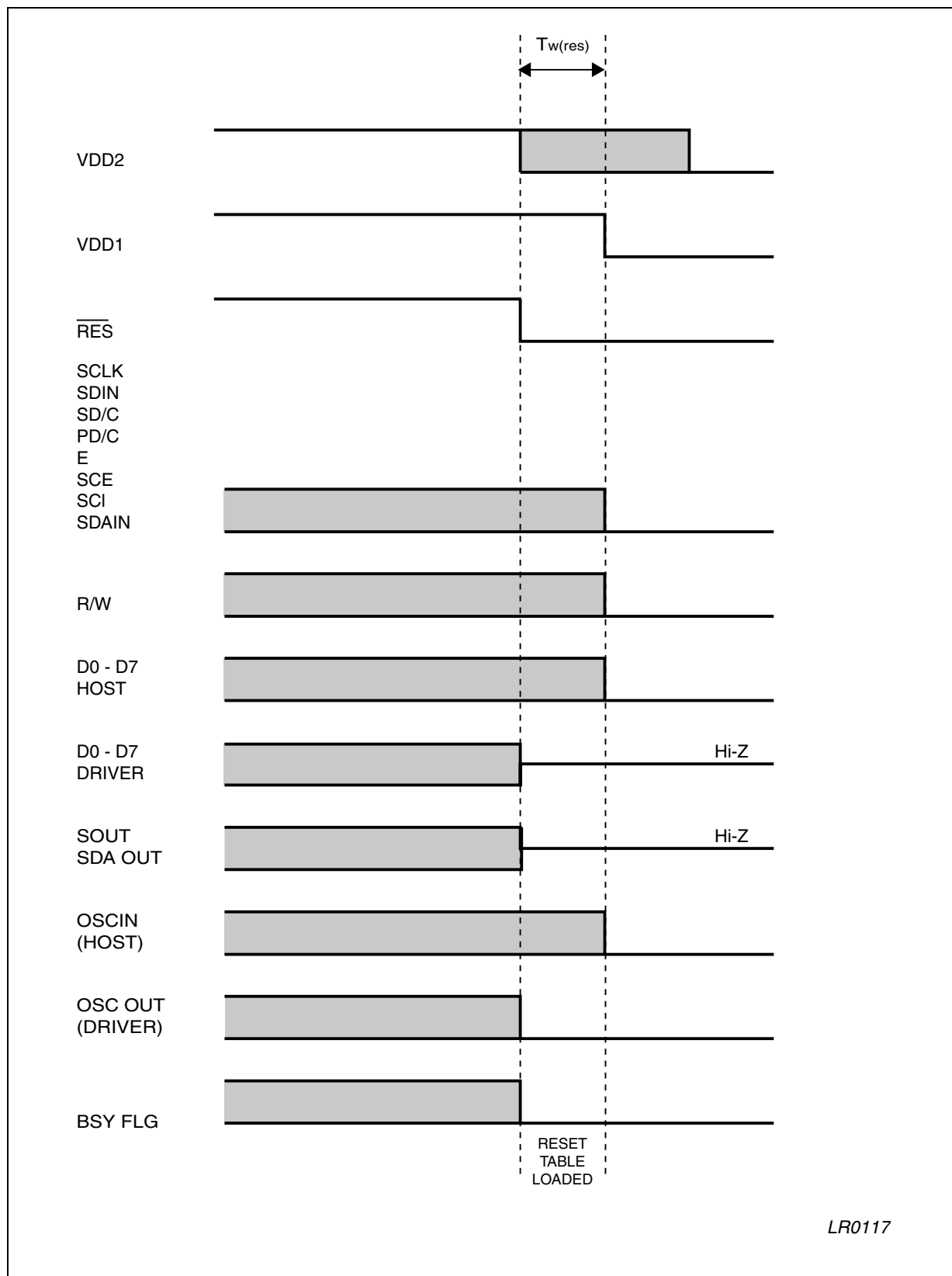
Figure 43. Power-OFF Sequence
