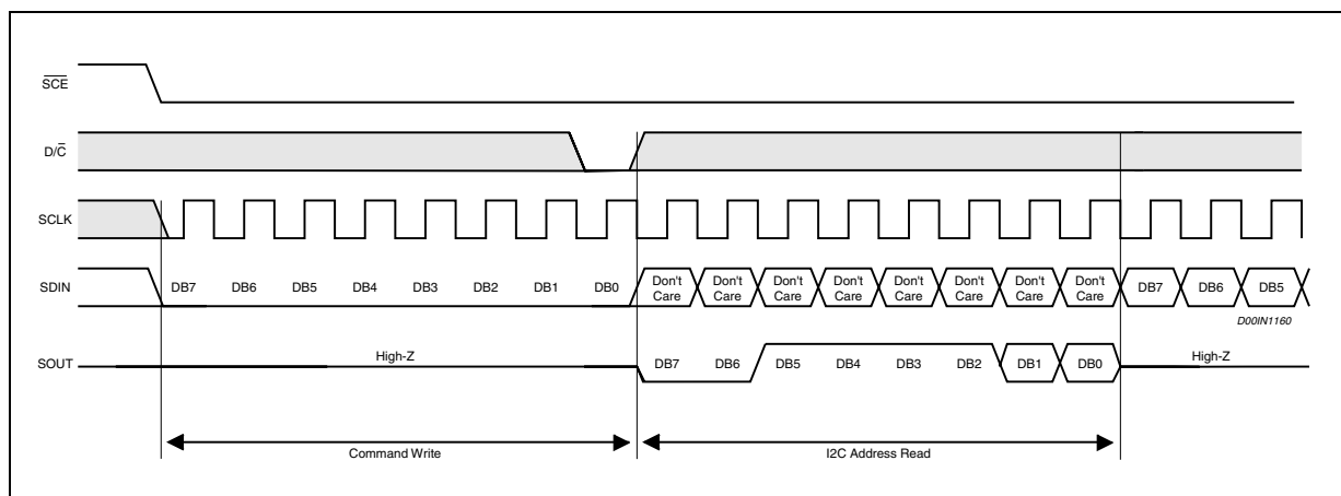
Figure 35. Reading Sequence
