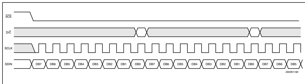
Figure 33. Serial bus protocol - several byte transmission
