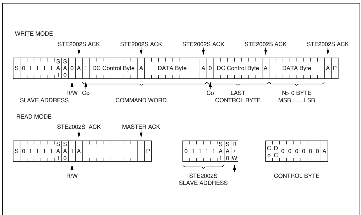
Figure 31. Communication Protocol
