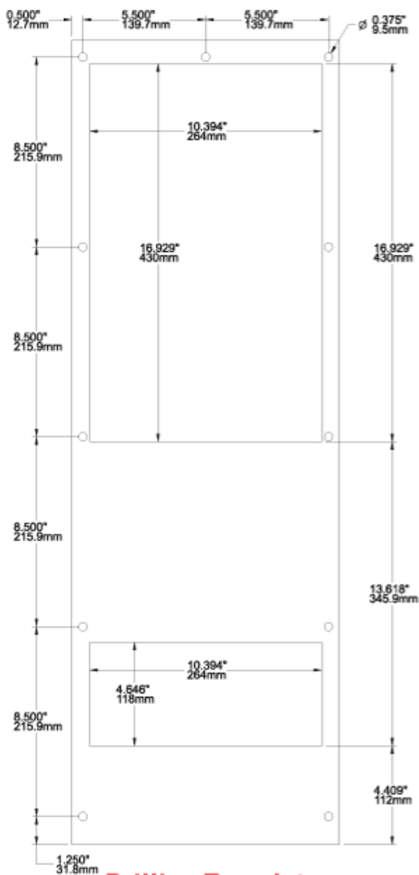
Drilling Template
